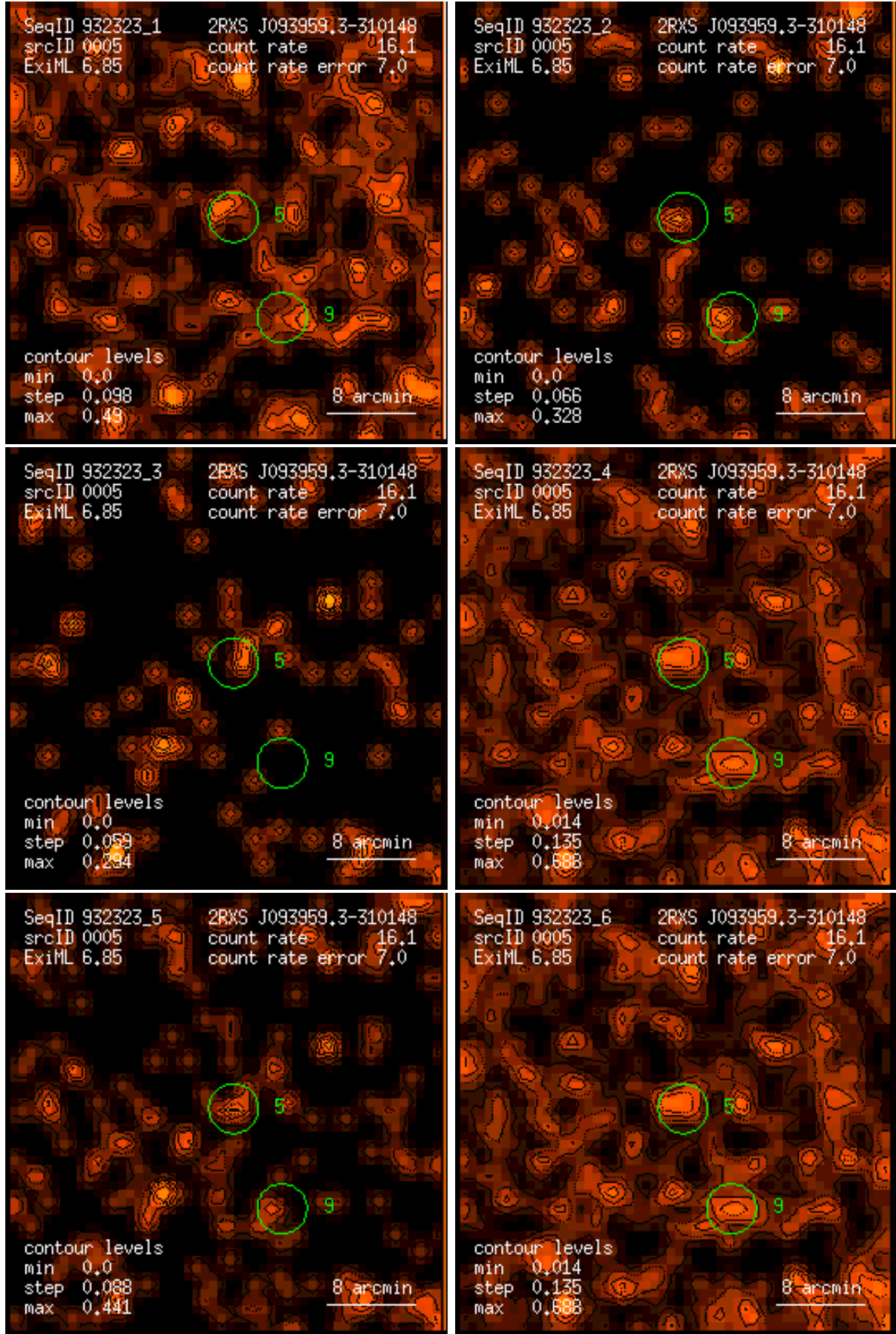
Figure 5: RASS 932323: detection 0005: band rate images, Gaussian filter: (1) PSPC channels 11 – 41, (2) 52 – 90, (3) 91 – 201, (4) 11 – 235, (5) 52 – 201, (6) 11 – 201. Broad band rates in counts/ks. Band rate contour levels in counts/ks/arcmin 2 .
