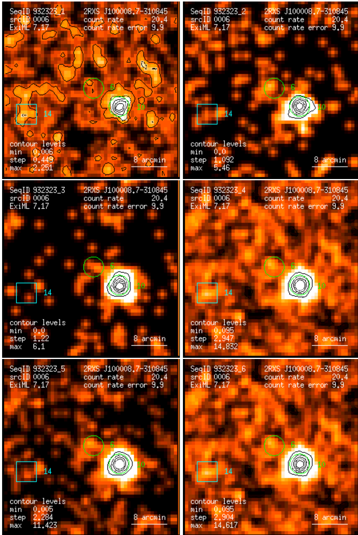
Figure 6: RASS 932323: detection 0006: band rate images, Gaussian filter: (1) PSPC channels 11 – 41, (2) 52 – 90, (3) 91 – 201, (4) 11 – 235, (5) 52 – 201, (6) 11 – 201. Broad band rates in counts/ks. Band rate contour levels in counts/ks/arcmin 2 .
