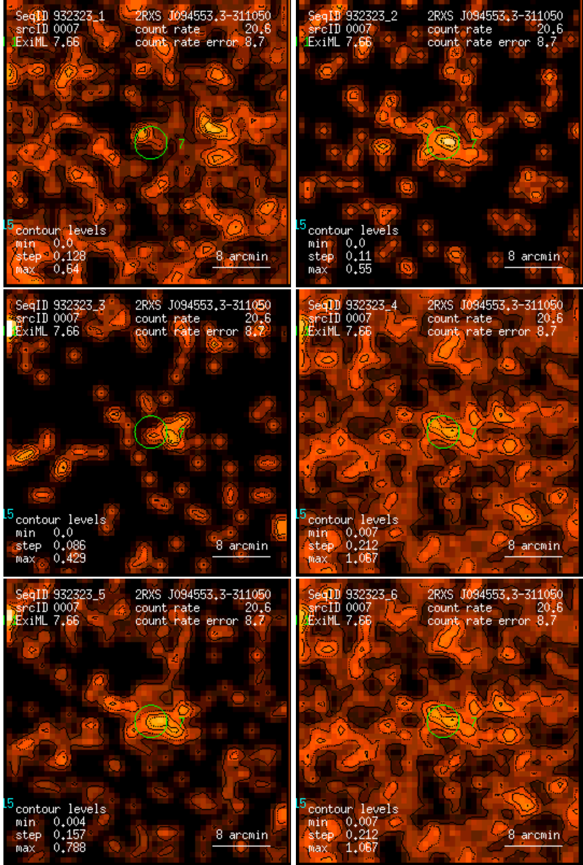
Figure 7: RASS 932323: detection 0007: band rate images, Gaussian filter: (1) PSPC channels 11 – 41, (2) 52 – 90, (3) 91 – 201, (4) 11 – 235, (5) 52 – 201, (6) 11 – 201. Broad band rates in counts/ks. Band rate contour levels in counts/ks/arcmin 2 .
