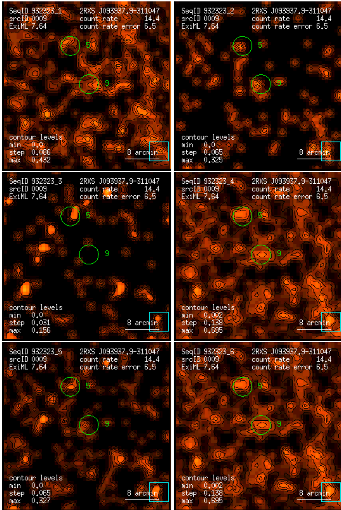
Figure 9: RASS 932323: detection 0009: band rate images, Gaussian filter: (1) PSPC channels 11 – 41, (2) 52 – 90, (3) 91 – 201, (4) 11 – 235, (5) 52 – 201, (6) 11 – 201. Broad band rates in counts/ks. Band rate contour levels in counts/ks/arcmin 2 .
