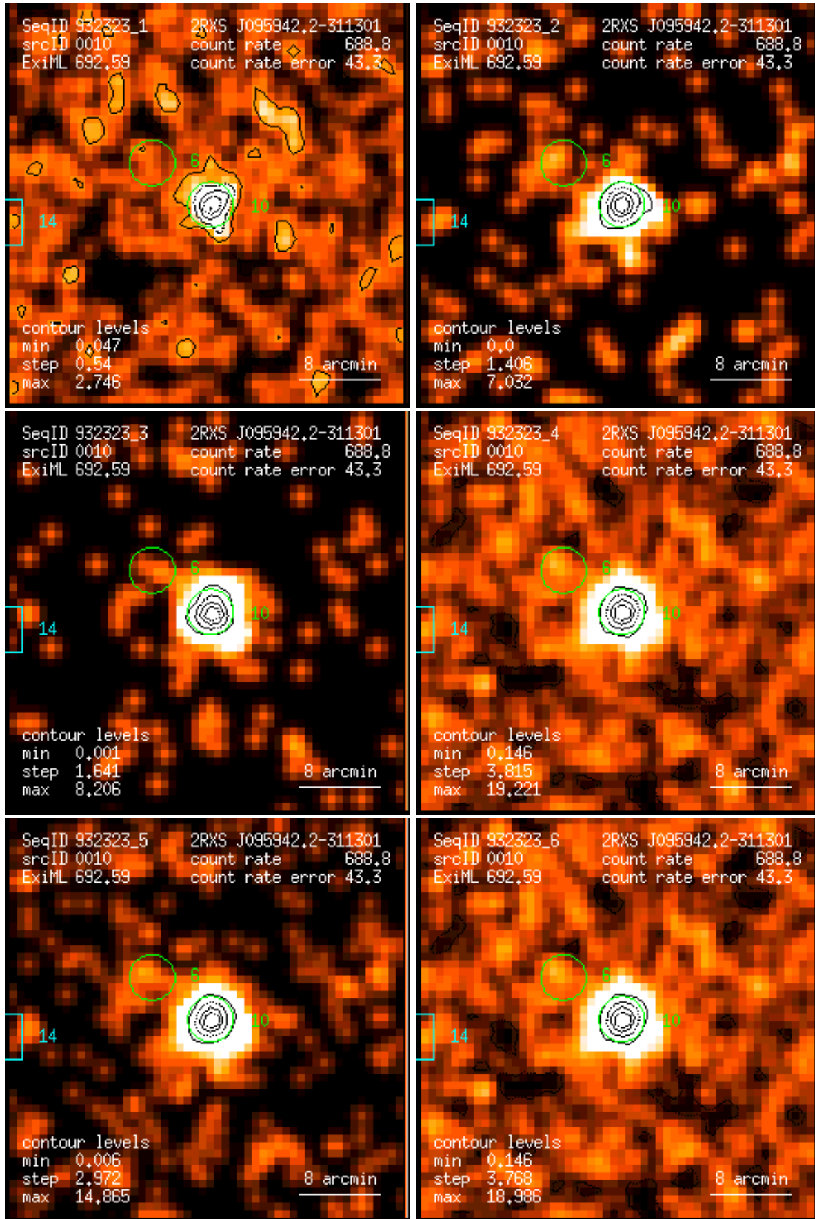
Figure 10: RASS 932323: detection 0010: band rate images, Gaussian filter: (1) PSPC channels 11 – 41, (2) 52 – 90, (3) 91 – 201, (4) 11 – 235, (5) 52 – 201, (6) 11 – 201. Broad band rates in counts/ks. Band rate contour levels in counts/ks/arcmin 2 .
