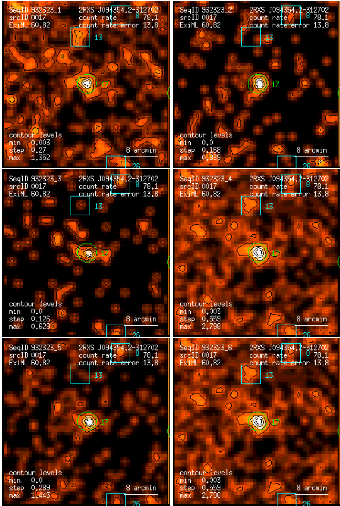
Figure 17: RASS 932323: detection 0017: band rate images, Gaussian filter: (1) PSPC channels 11 – 41, (2) 52 – 90, (3) 91 – 201, (4) 11 – 235, (5) 52 – 201, (6) 11 – 201. Broad band rates in counts/ks. Band rate contour levels in counts/ks/arcmin 2 .
