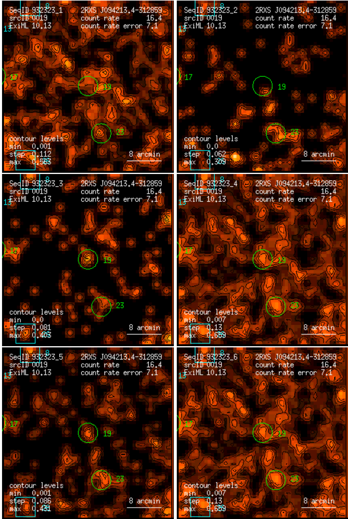
Figure 19: RASS 932323: detection 0019: band rate images, Gaussian filter: (1) PSPC channels 11 – 41, (2) 52 – 90, (3) 91 – 201, (4) 11 – 235, (5) 52 – 201, (6) 11 – 201. Broad band rates in counts/ks. Band rate contour levels in counts/ks/arcmin 2 .
