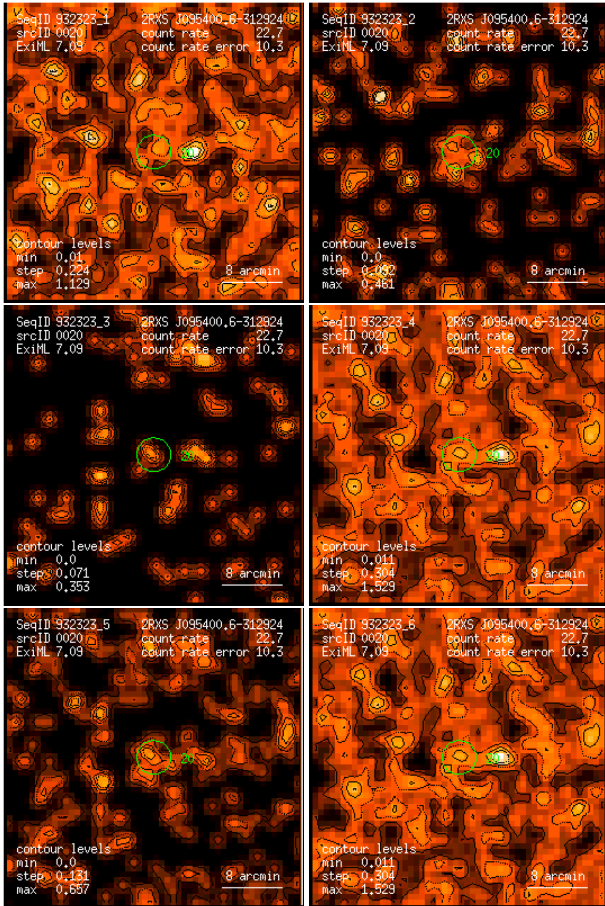
Figure 20: RASS 932323: detection 0020: band rate images, Gaussian filter: (1) PSPC channels 11 – 41, (2) 52 – 90, (3) 91 – 201, (4) 11 – 235, (5) 52 – 201, (6) 11 – 201. Broad band rates in counts/ks. Band rate contour levels in counts/ks/arcmin 2 .
