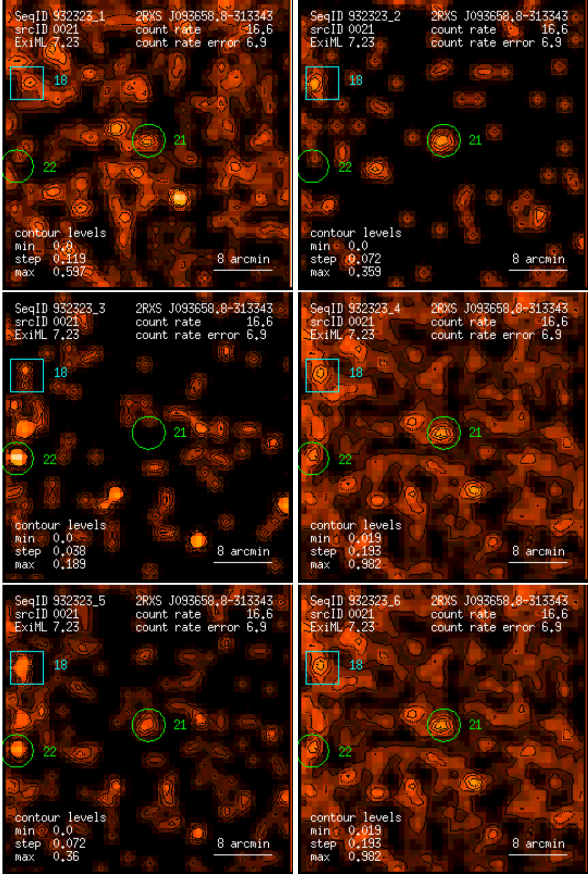
Figure 21: RASS 932323: detection 0021: band rate images, Gaussian filter: (1) PSPC channels 11 – 41, (2) 52 – 90, (3) 91 – 201, (4) 11 – 235, (5) 52 – 201, (6) 11 – 201. Broad band rates in counts/ks. Band rate contour levels in counts/ks/arcmin 2 .
