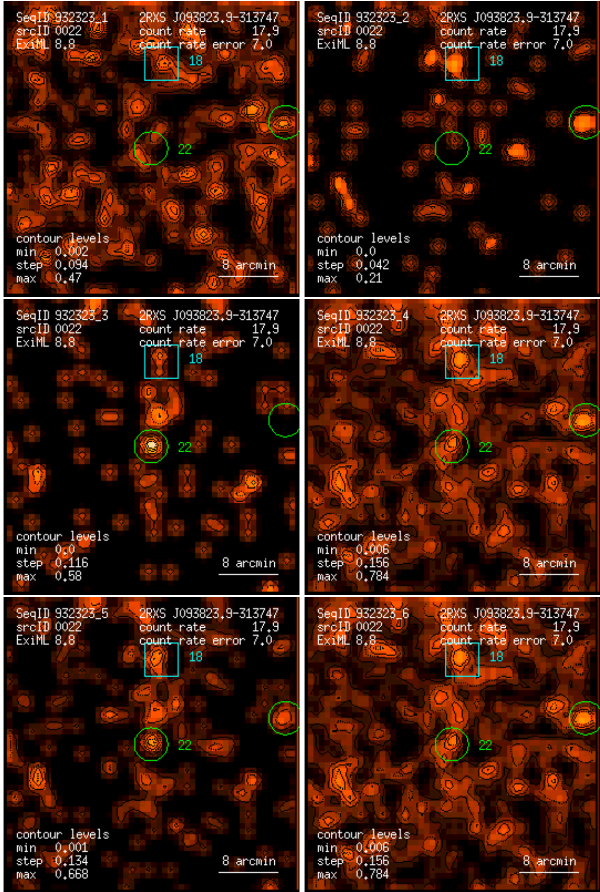
Figure 22: RASS 932323: detection 0022: band rate images, Gaussian filter: (1) PSPC channels 11 – 41, (2) 52 – 90, (3) 91 – 201, (4) 11 – 235, (5) 52 – 201, (6) 11 – 201. Broad band rates in counts/ks. Band rate contour levels in counts/ks/arcmin 2 .
