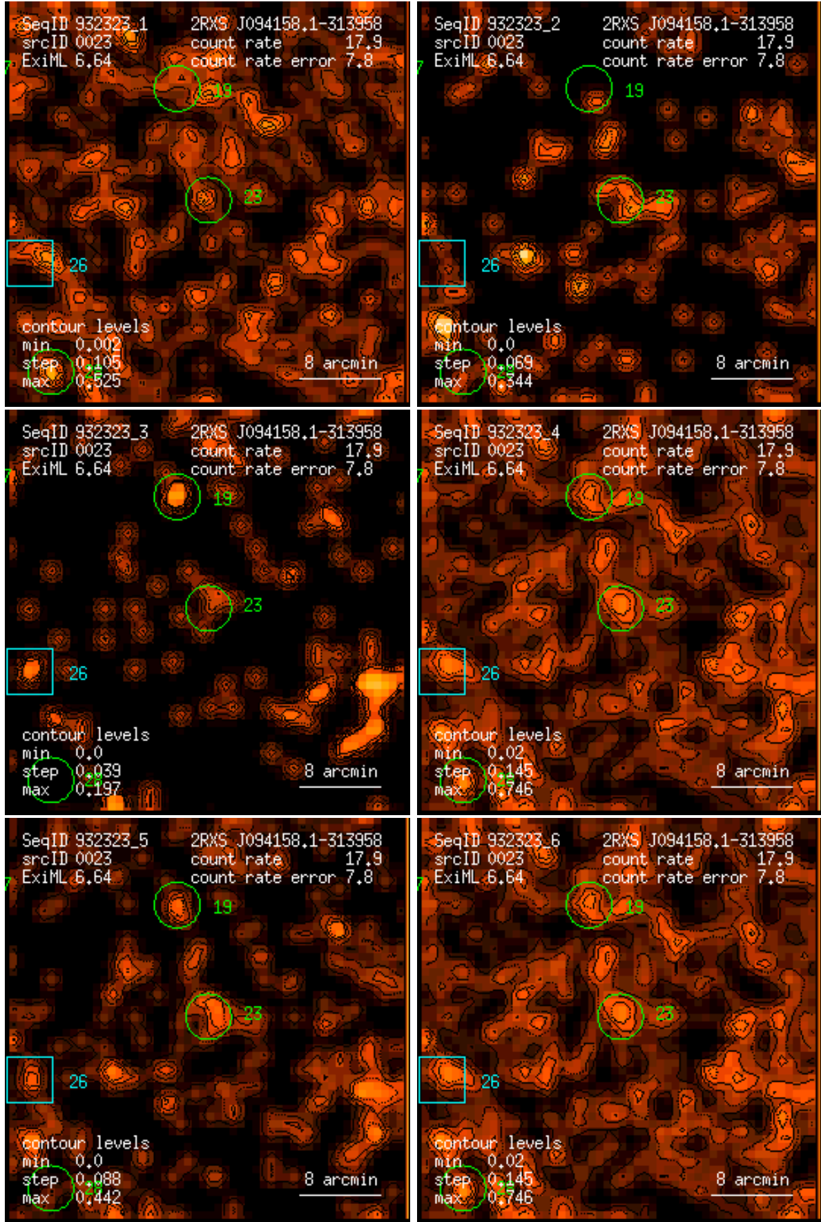
Figure 23: RASS 932323: detection 0023: band rate images, Gaussian filter: (1) PSPC channels 11 – 41, (2) 52 – 90, (3) 91 – 201, (4) 11 – 235, (5) 52 – 201, (6) 11 – 201. Broad band rates in counts/ks. Band rate contour levels in counts/ks/arcmin 2 .
