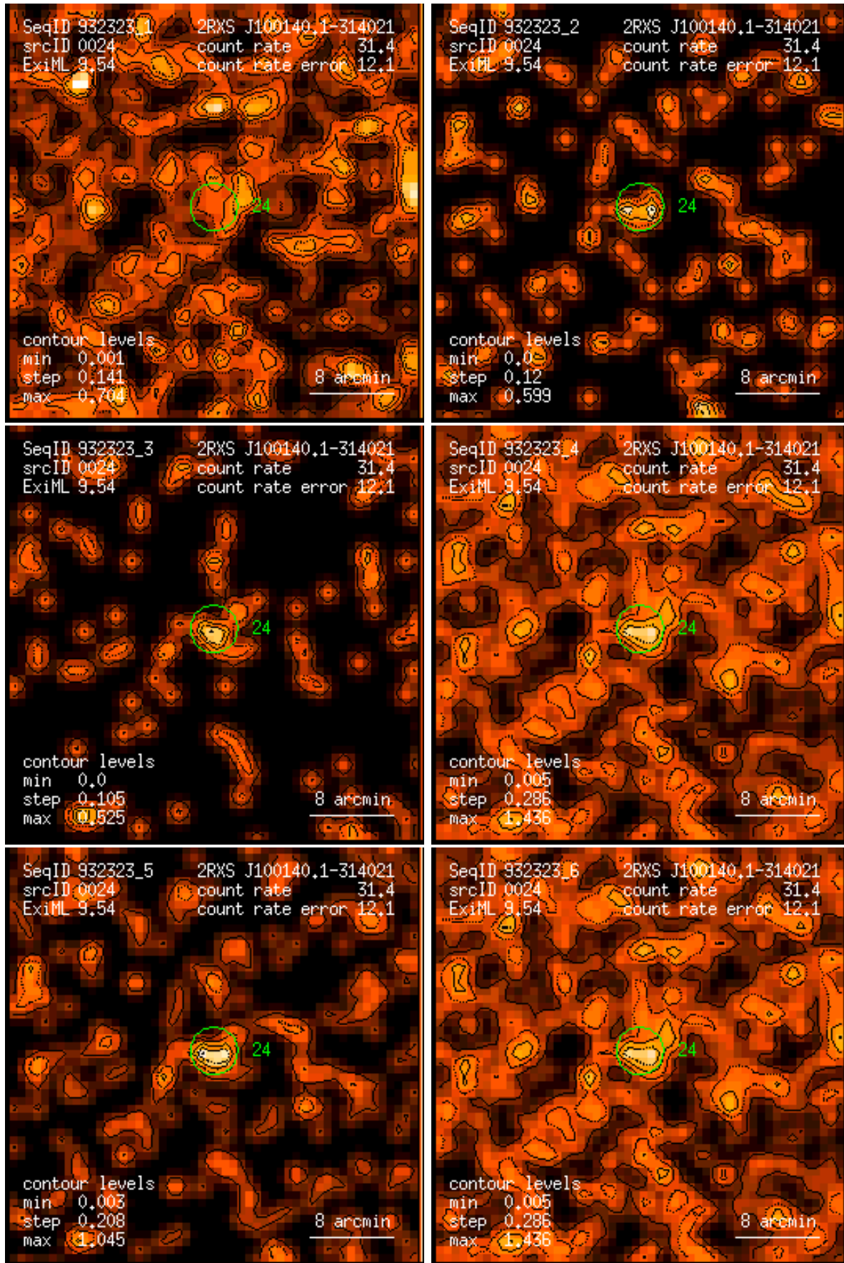
Figure 24: RASS 932323: detection 0024: band rate images, Gaussian filter: (1) PSPC channels 11 – 41, (2) 52 – 90, (3) 91 – 201, (4) 11 – 235, (5) 52 – 201, (6) 11 – 201. Broad band rates in counts/ks. Band rate contour levels in counts/ks/arcmin 2 .
