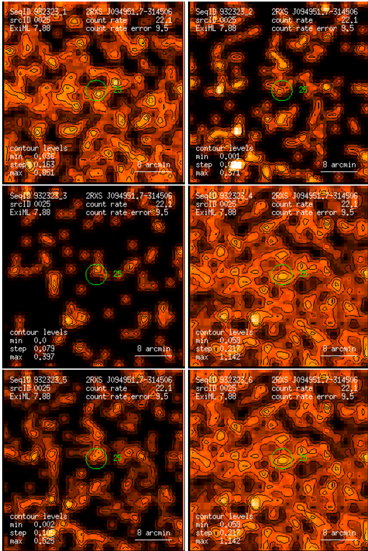
Figure 25: RASS 932323: detection 0025: band rate images, Gaussian filter: (1) PSPC channels 11 – 41, (2) 52 – 90, (3) 91 – 201, (4) 11 – 235, (5) 52 – 201, (6) 11 – 201. Broad band rates in counts/ks. Band rate contour levels in counts/ks/arcmin 2 .
