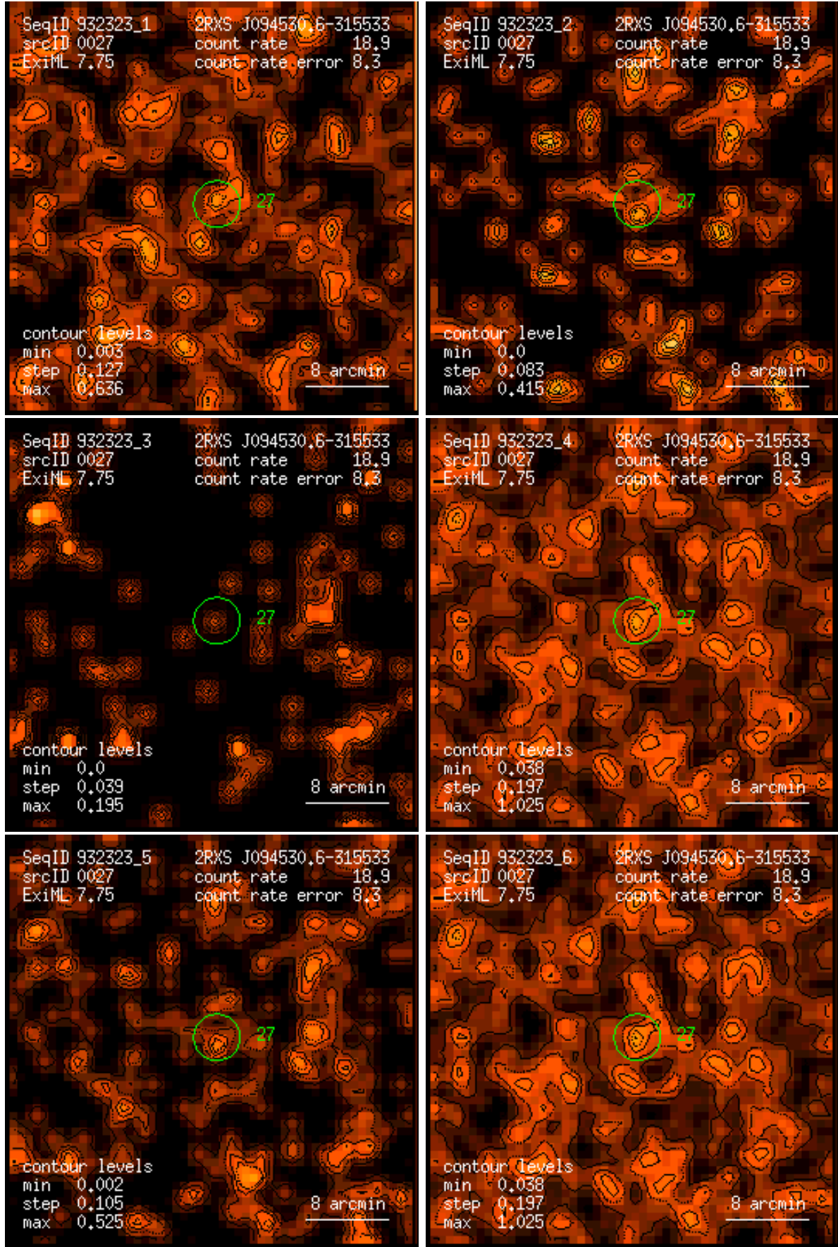
Figure 27: RASS 932323: detection 0027: band rate images, Gaussian filter: (1) PSPC channels 11 – 41, (2) 52 – 90, (3) 91 – 201, (4) 11 – 235, (5) 52 – 201, (6) 11 – 201. Broad band rates in counts/ks. Band rate contour levels in counts/ks/arcmin 2 .
