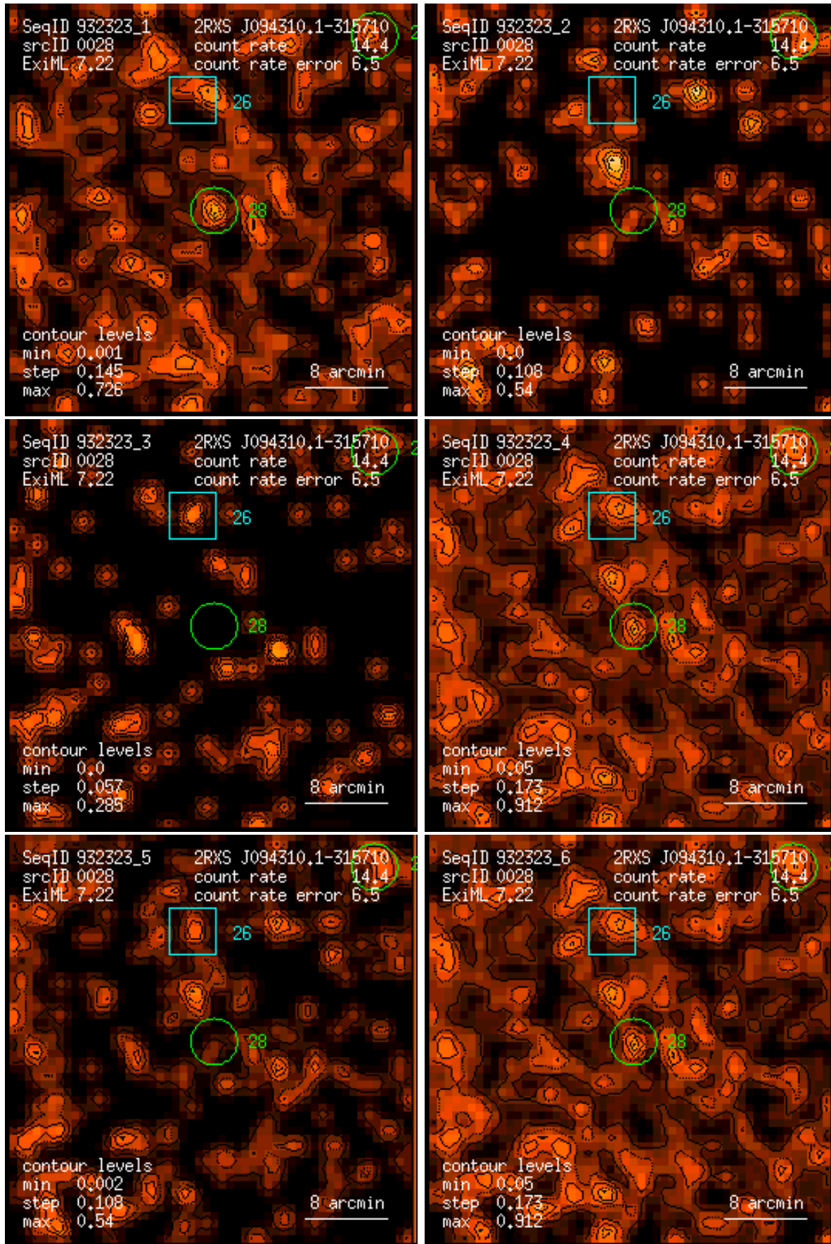
Figure 28: RASS 932323: detection 0028: band rate images, Gaussian filter: (1) PSPC channels 11 – 41, (2) 52 – 90, (3) 91 – 201, (4) 11 – 235, (5) 52 – 201, (6) 11 – 201. Broad band rates in counts/ks. Band rate contour levels in counts/ks/arcmin 2 .
