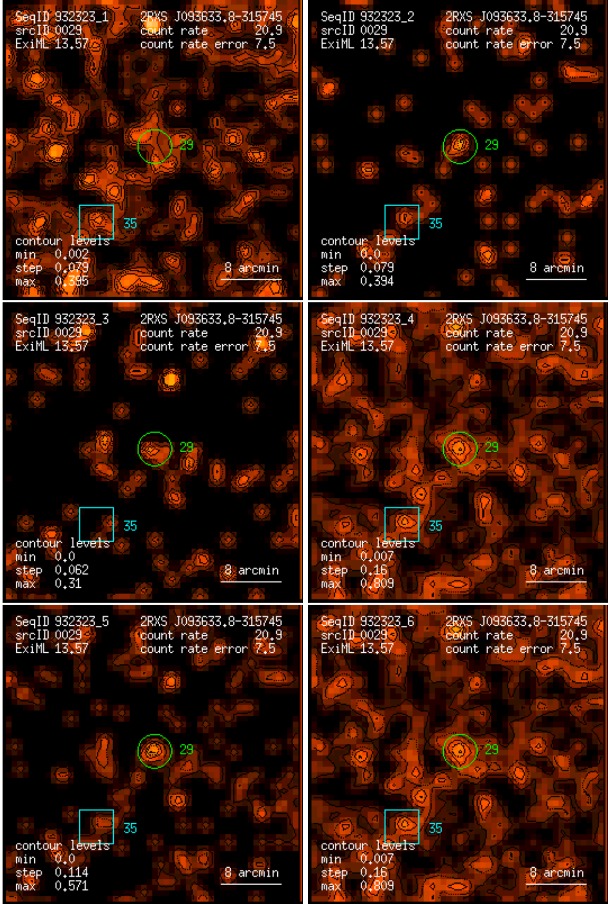
Figure 29: RASS 932323: detection 0029: band rate images, Gaussian filter: (1) PSPC channels 11 – 41, (2) 52 – 90, (3) 91 – 201, (4) 11 – 235, (5) 52 – 201, (6) 11 – 201. Broad band rates in counts/ks. Band rate contour levels in counts/ks/arcmin 2 .
