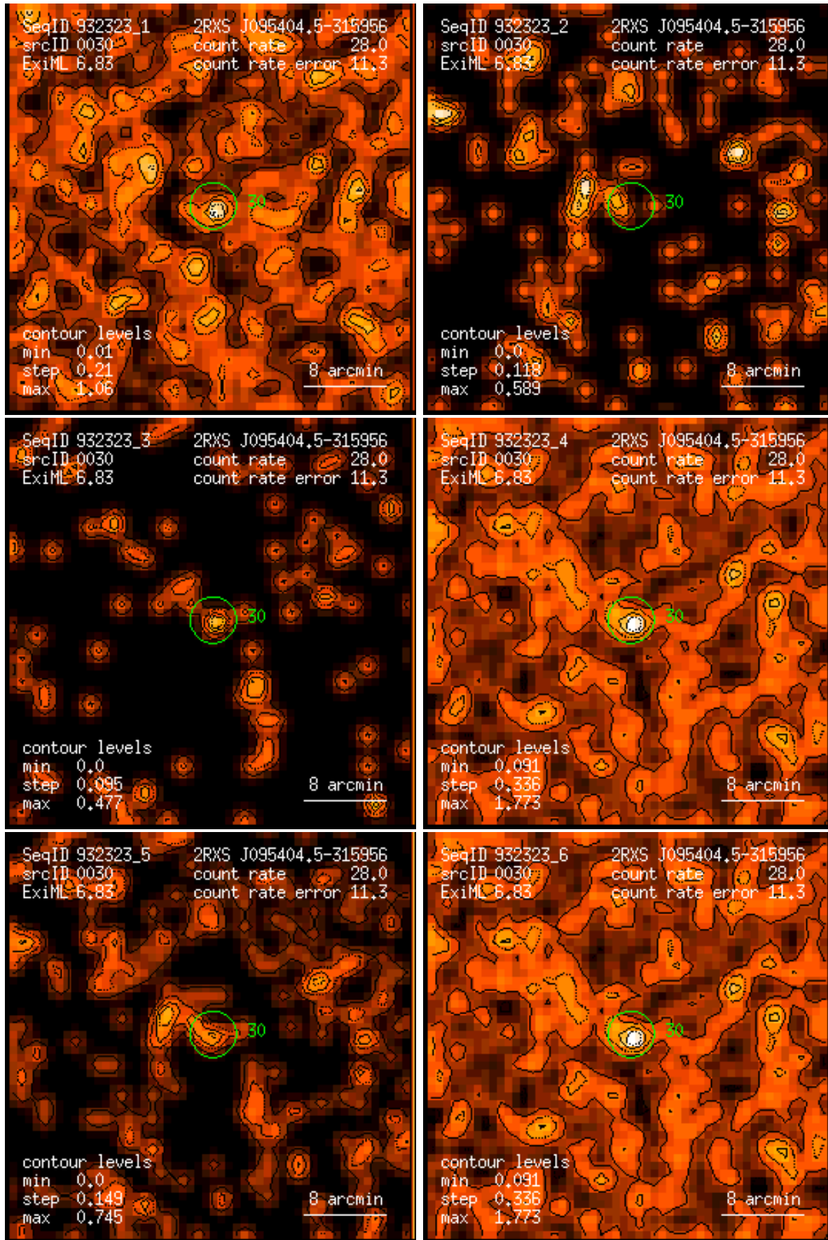
Figure 30: RASS 932323: detection 0030: band rate images, Gaussian filter: (1) PSPC channels 11 – 41, (2) 52 – 90, (3) 91 – 201, (4) 11 – 235, (5) 52 – 201, (6) 11 – 201. Broad band rates in counts/ks. Band rate contour levels in counts/ks/arcmin 2 .
