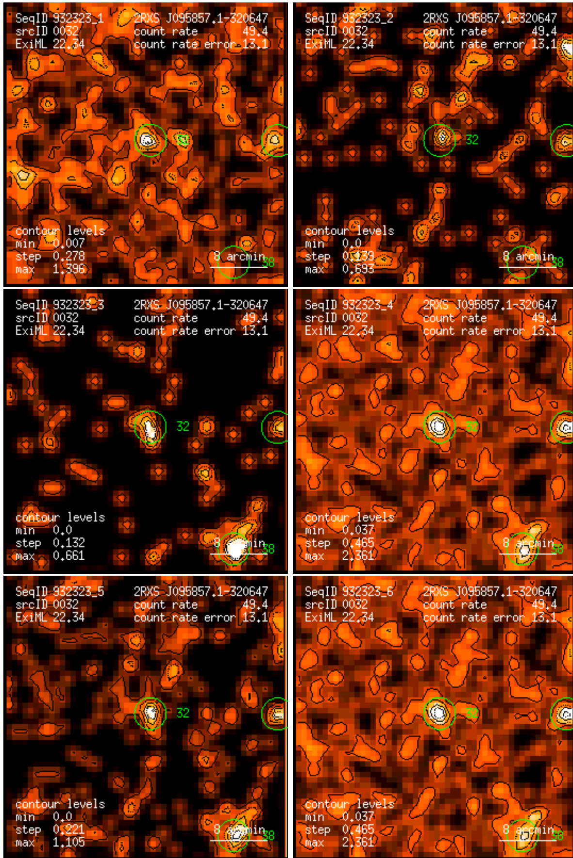
Figure 32: RASS 932323: detection 0032: band rate images, Gaussian filter: (1) PSPC channels 11 – 41, (2) 52 – 90, (3) 91 – 201, (4) 11 – 235, (5) 52 – 201, (6) 11 – 201. Broad band rates in counts/ks. Band rate contour levels in counts/ks/arcmin 2 .
