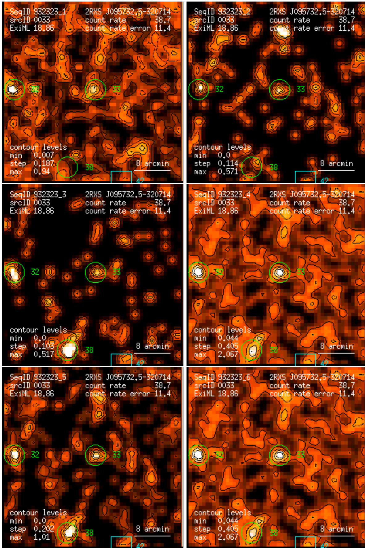
Figure 33: RASS 932323: detection 0033: band rate images, Gaussian filter: (1) PSPC channels 11 – 41, (2) 52 – 90, (3) 91 – 201, (4) 11 – 235, (5) 52 – 201, (6) 11 – 201. Broad band rates in counts/ks. Band rate contour levels in counts/ks/arcmin 2 .
