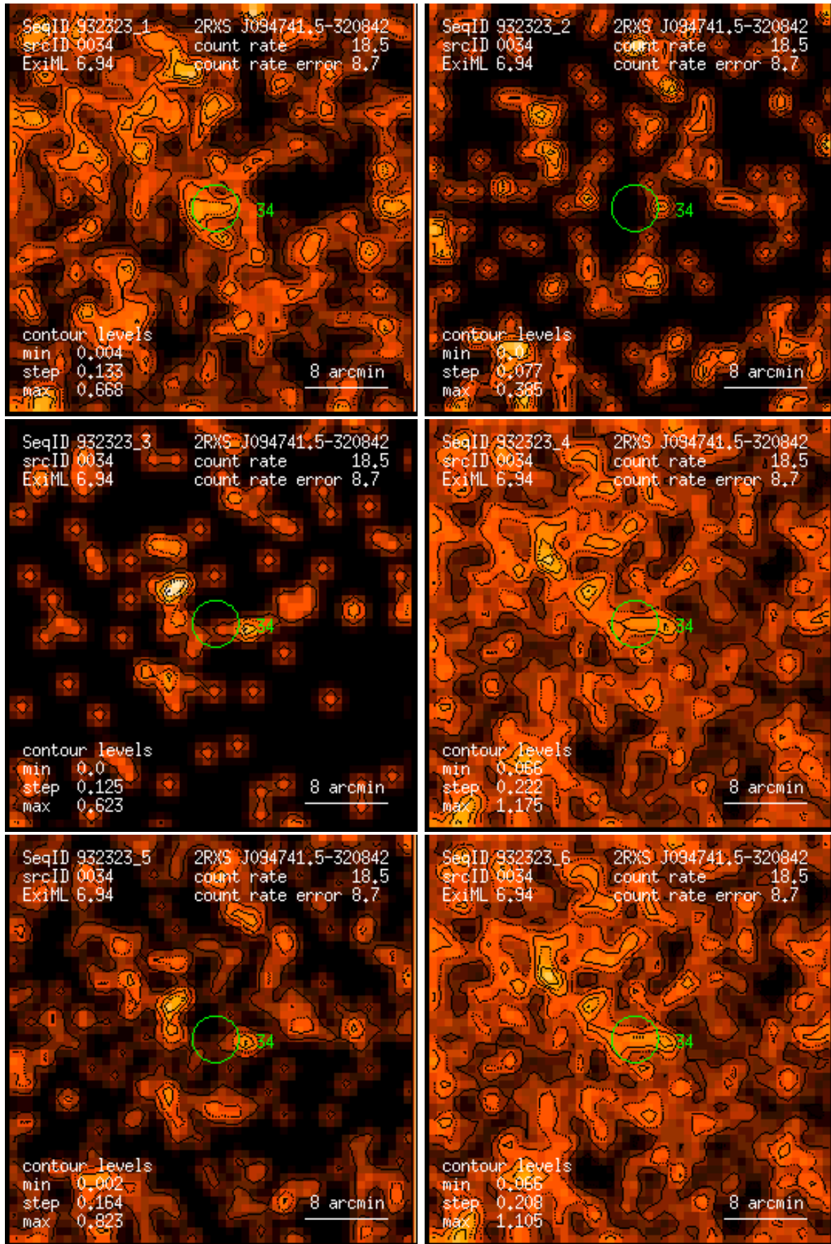
Figure 34: RASS 932323: detection 0034: band rate images, Gaussian filter: (1) PSPC channels 11 – 41, (2) 52 – 90, (3) 91 – 201, (4) 11 – 235, (5) 52 – 201, (6) 11 – 201. Broad band rates in counts/ks. Band rate contour levels in counts/ks/arcmin 2 .
