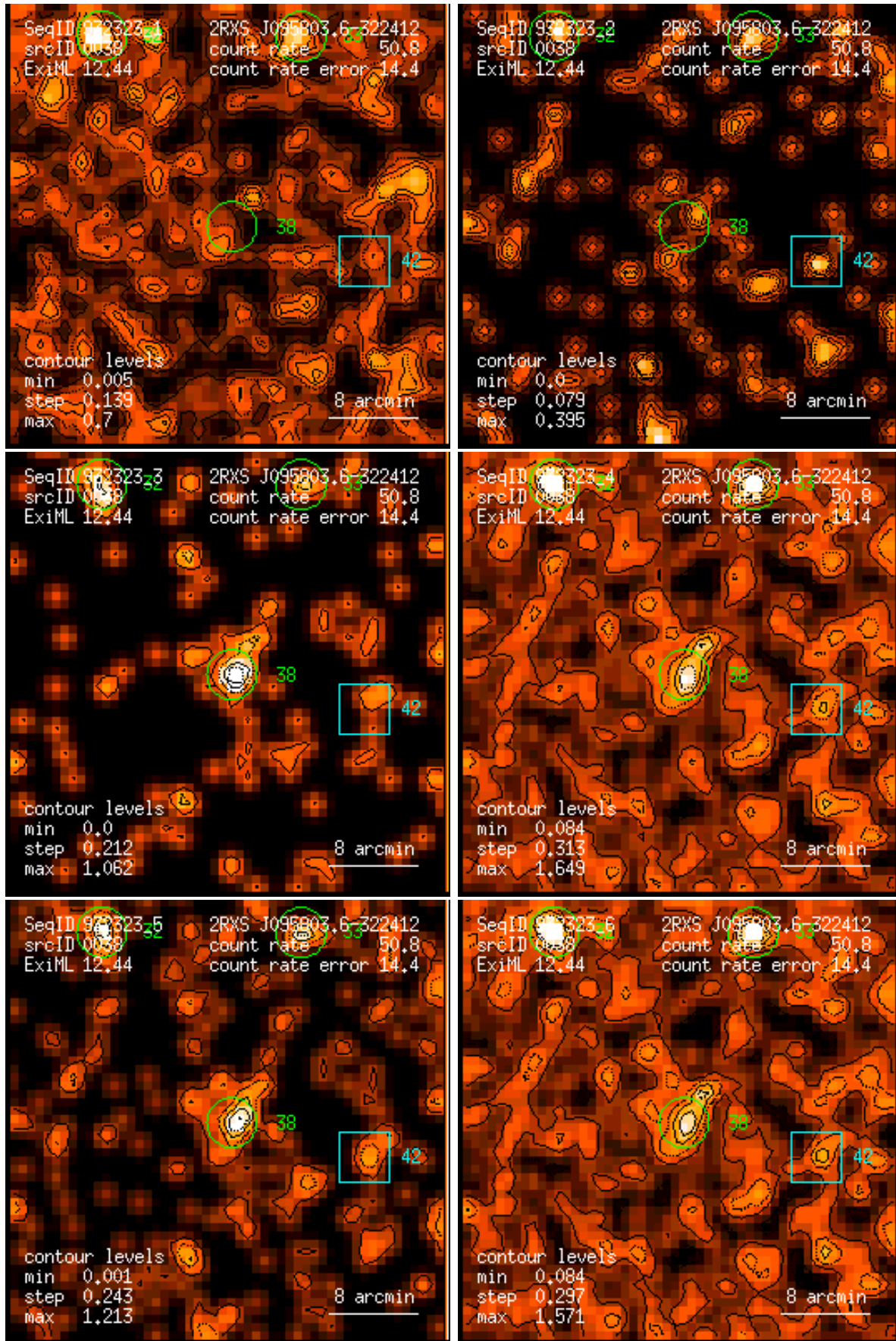
Figure 38: RASS 932323: detection 0038: band rate images, Gaussian filter: (1) PSPC channels 11 – 41, (2) 52 – 90, (3) 91 – 201, (4) 11 – 235, (5) 52 – 201, (6) 11 – 201. Broad band rates in counts/ks. Band rate contour levels in counts/ks/arcmin 2 .
