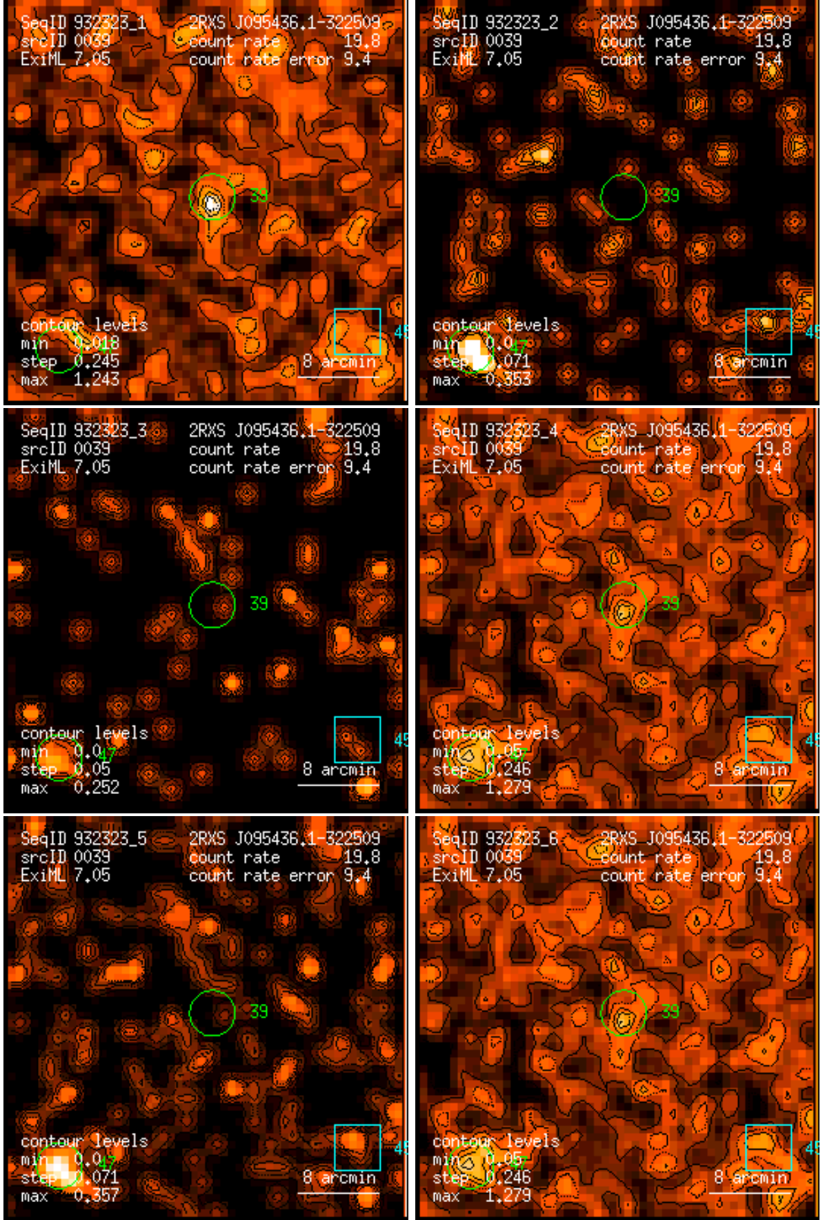
Figure 39: RASS 932323: detection 0039: band rate images, Gaussian filter: (1) PSPC channels 11 – 41, (2) 52 – 90, (3) 91 – 201, (4) 11 – 235, (5) 52 – 201, (6) 11 – 201. Broad band rates in counts/ks. Band rate contour levels in counts/ks/arcmin 2 .
