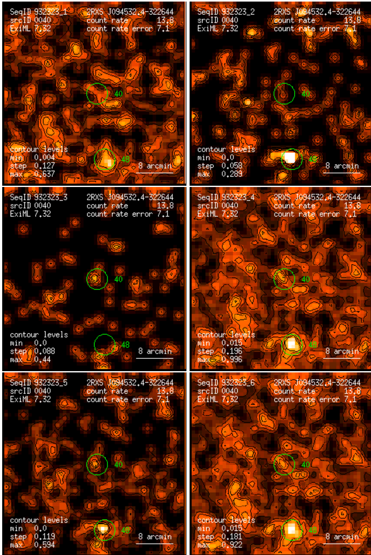
Figure 40: RASS 932323: detection 0040: band rate images, Gaussian filter: (1) PSPC channels 11 – 41, (2) 52 – 90, (3) 91 – 201, (4) 11 – 235, (5) 52 – 201, (6) 11 – 201. Broad band rates in counts/ks. Band rate contour levels in counts/ks/arcmin 2 .
