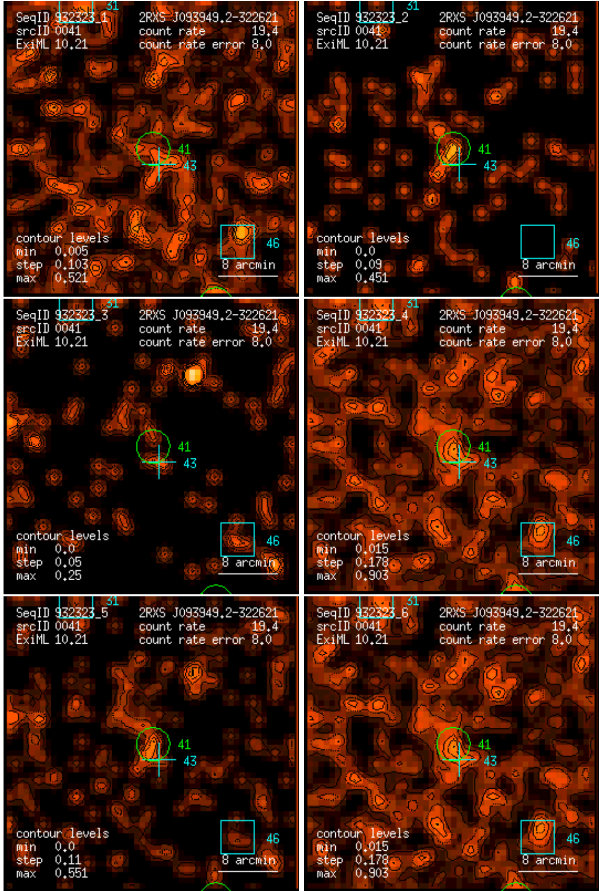
Figure 41: RASS 932323: detection 0041: band rate images, Gaussian filter: (1) PSPC channels 11 – 41, (2) 52 – 90, (3) 91 – 201, (4) 11 – 235, (5) 52 – 201, (6) 11 – 201. Broad band rates in counts/ks. Band rate contour levels in counts/ks/arcmin 2 .
