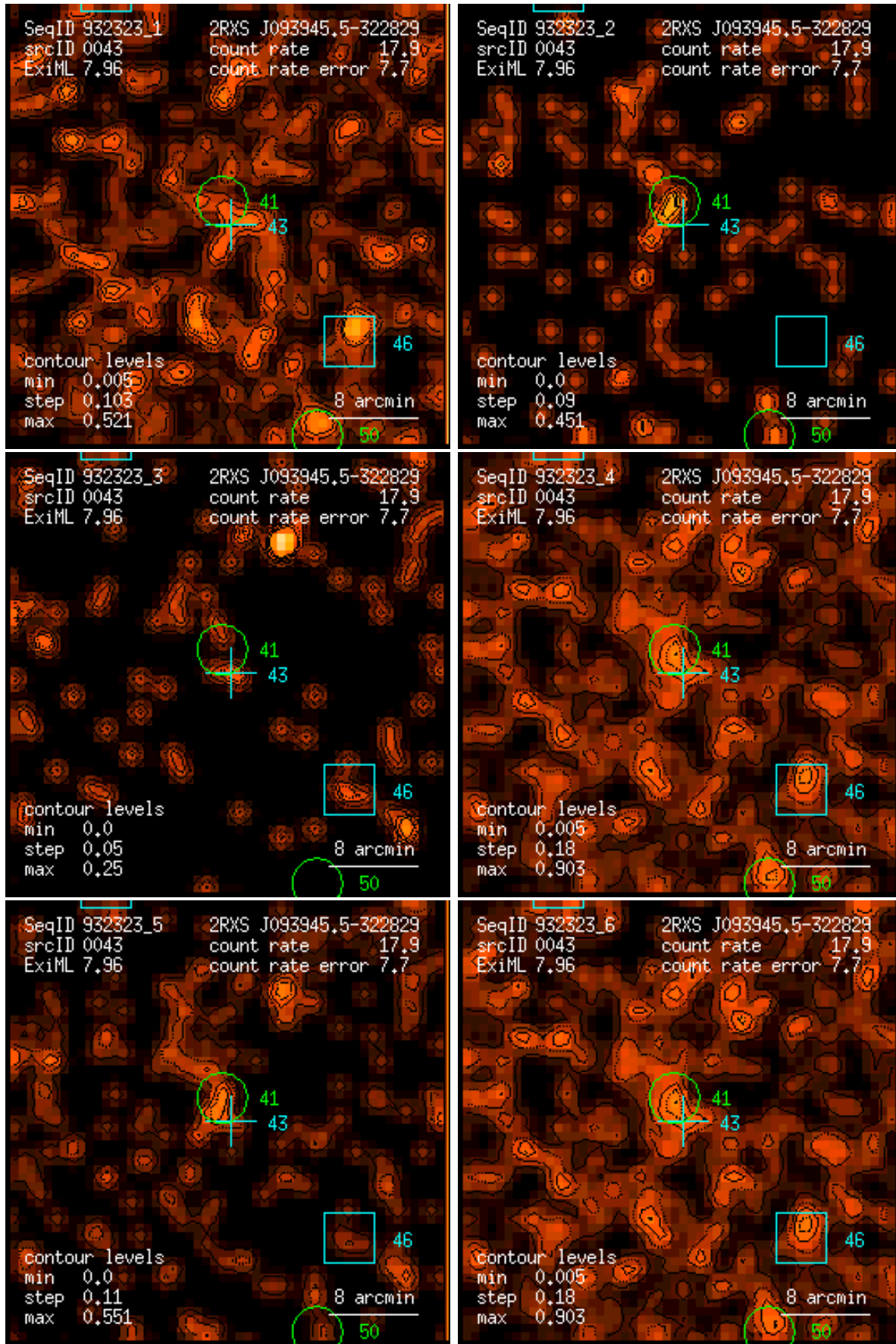
Figure 43: RASS 932323: detection 0043: band rate images, Gaussian filter: (1) PSPC channels 11 – 41, (2) 52 – 90, (3) 91 – 201, (4) 11 – 235, (5) 52 – 201, (6) 11 – 201. Broad band rates in counts/ks. Band rate contour levels in counts/ks/arcmin 2 .
