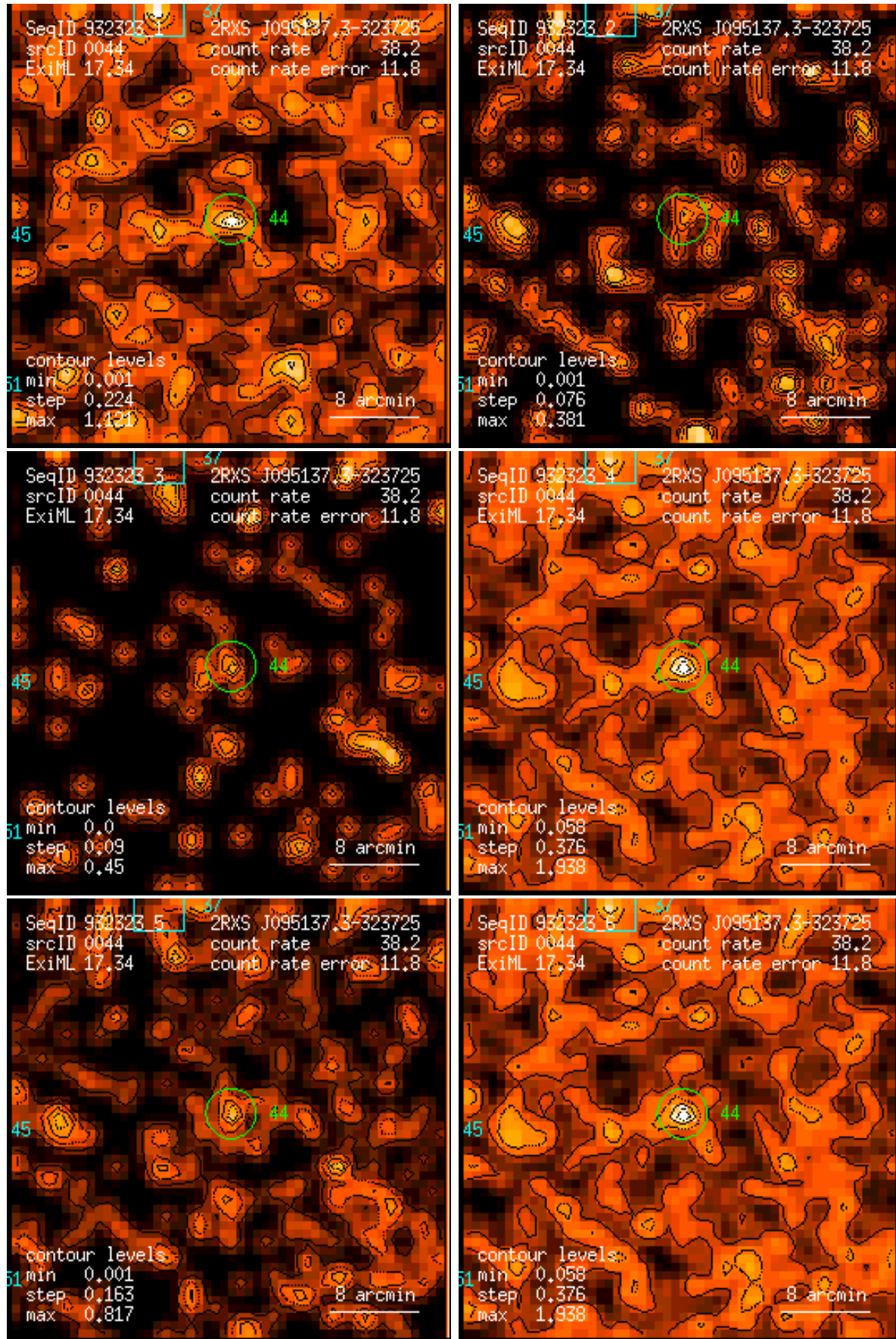
Figure 44: RASS 932323: detection 0044: band rate images, Gaussian filter: (1) PSPC channels 11 – 41, (2) 52 – 90, (3) 91 – 201, (4) 11 – 235, (5) 52 – 201, (6) 11 – 201. Broad band rates in counts/ks. Band rate contour levels in counts/ks/arcmin 2 .
