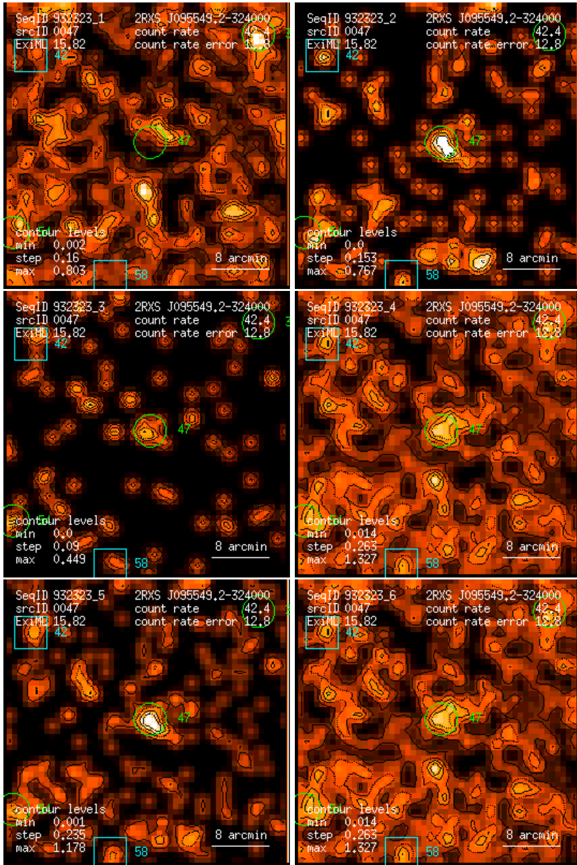
Figure 47: RASS 932323: detection 0047: band rate images, Gaussian filter: (1) PSPC channels 11 – 41, (2) 52 – 90, (3) 91 – 201, (4) 11 – 235, (5) 52 – 201, (6) 11 – 201. Broad band rates in counts/ks. Band rate contour levels in counts/ks/arcmin 2 .
