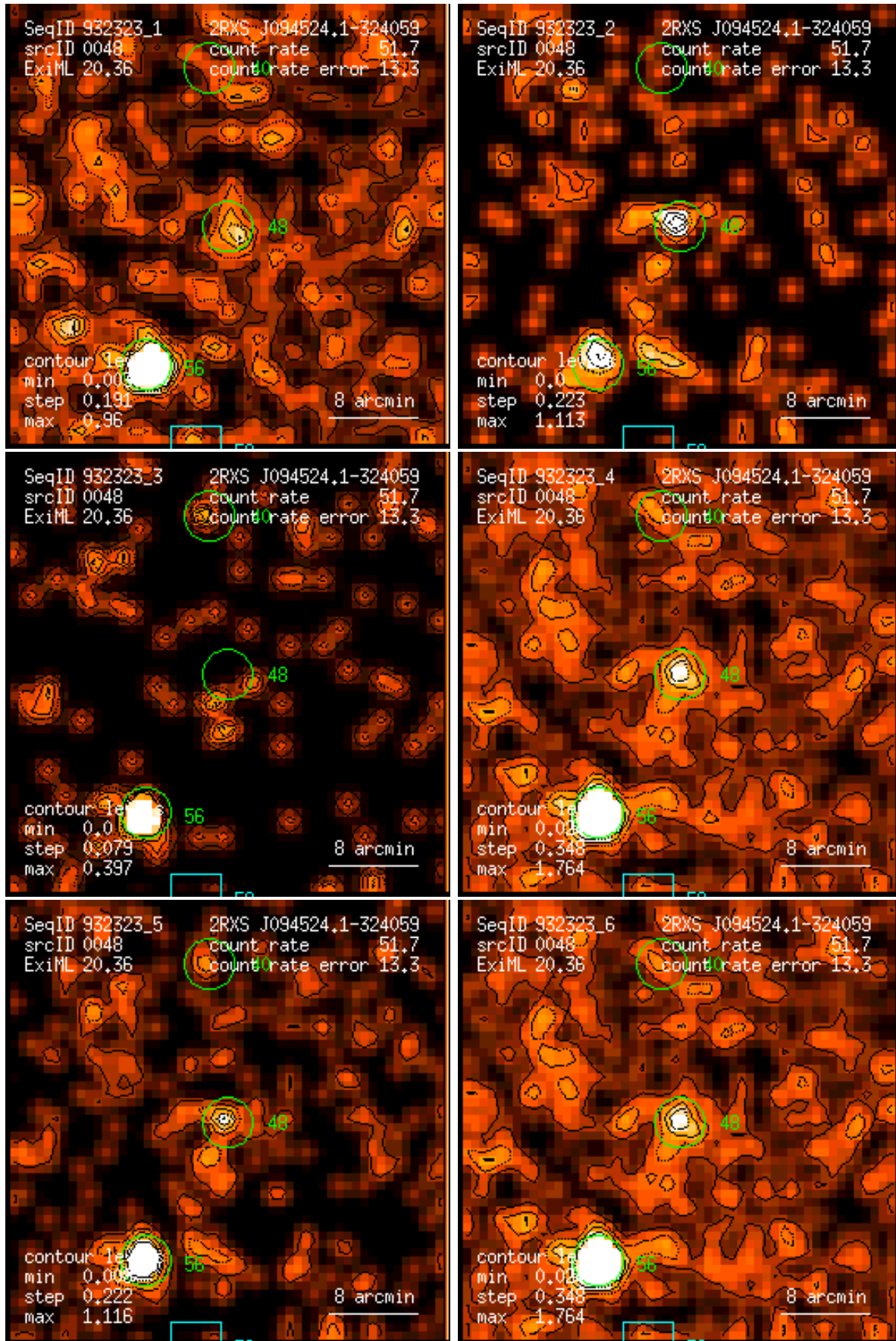
Figure 48: RASS 932323: detection 0048: band rate images, Gaussian filter: (1) PSPC channels 11 – 41, (2) 52 – 90, (3) 91 – 201, (4) 11 – 235, (5) 52 – 201, (6) 11 – 201. Broad band rates in counts/ks. Band rate contour levels in counts/ks/arcmin 2 .
