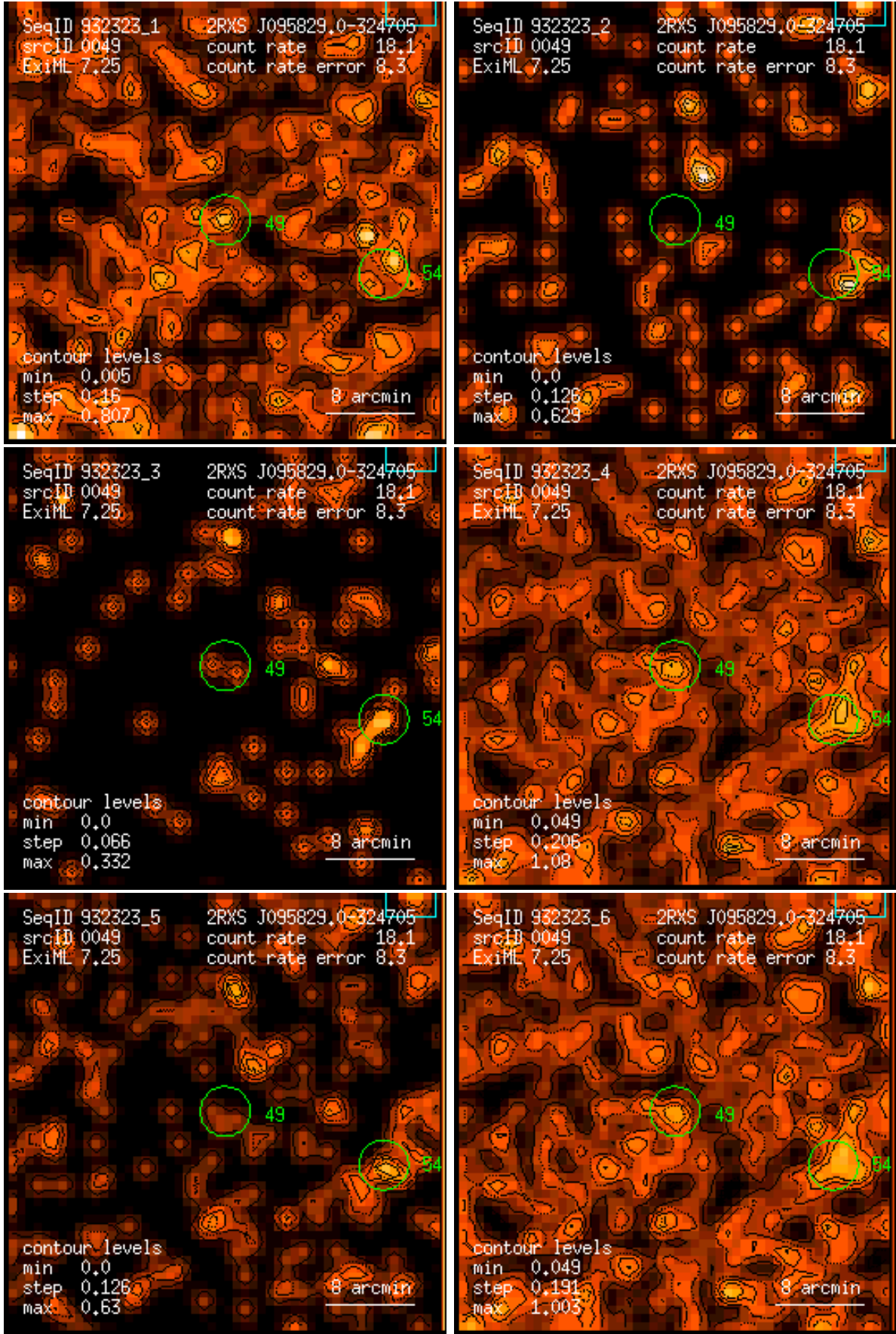
Figure 49: RASS 932323: detection 0049: band rate images, Gaussian filter: (1) PSPC channels 11 – 41, (2) 52 – 90, (3) 91 – 201, (4) 11 – 235, (5) 52 – 201, (6) 11 – 201. Broad band rates in counts/ks. Band rate contour levels in counts/ks/arcmin 2 .
