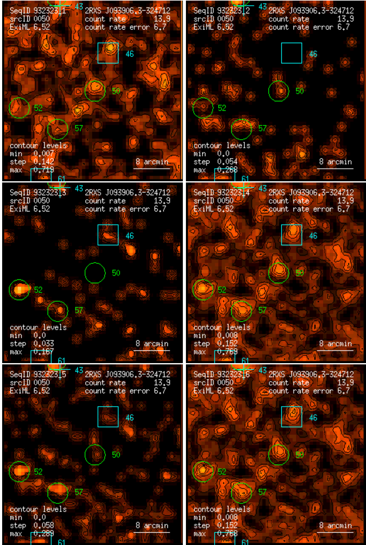
Figure 50: RASS 932323: detection 0050: band rate images, Gaussian filter: (1) PSPC channels 11 – 41, (2) 52 – 90, (3) 91 – 201, (4) 11 – 235, (5) 52 – 201, (6) 11 – 201. Broad band rates in counts/ks. Band rate contour levels in counts/ks/arcmin 2 .
