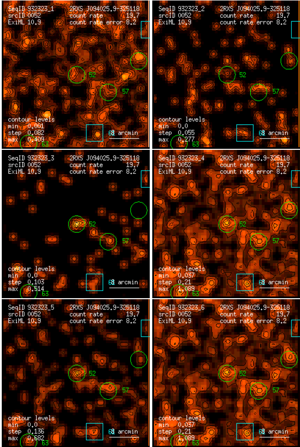
Figure 52: RASS 932323: detection 0052: band rate images, Gaussian filter: (1) PSPC channels 11 – 41, (2) 52 – 90, (3) 91 – 201, (4) 11 – 235, (5) 52 – 201, (6) 11 – 201. Broad band rates in counts/ks. Band rate contour levels in counts/ks/arcmin 2 .
