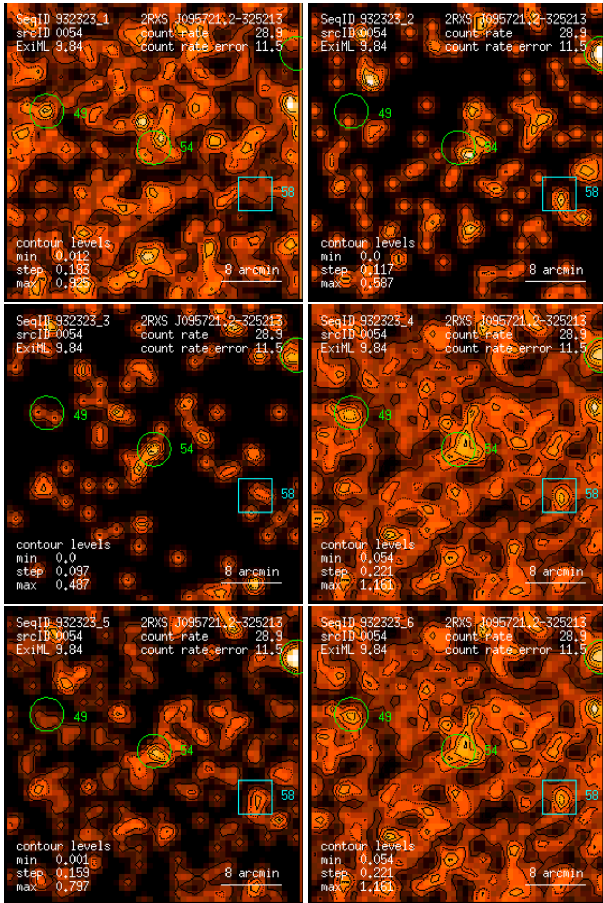
Figure 54: RASS 932323: detection 0054: band rate images, Gaussian filter: (1) PSPC channels 11 – 41, (2) 52 – 90, (3) 91 – 201, (4) 11 – 235, (5) 52 – 201, (6) 11 – 201. Broad band rates in counts/ks. Band rate contour levels in counts/ks/arcmin 2 .
