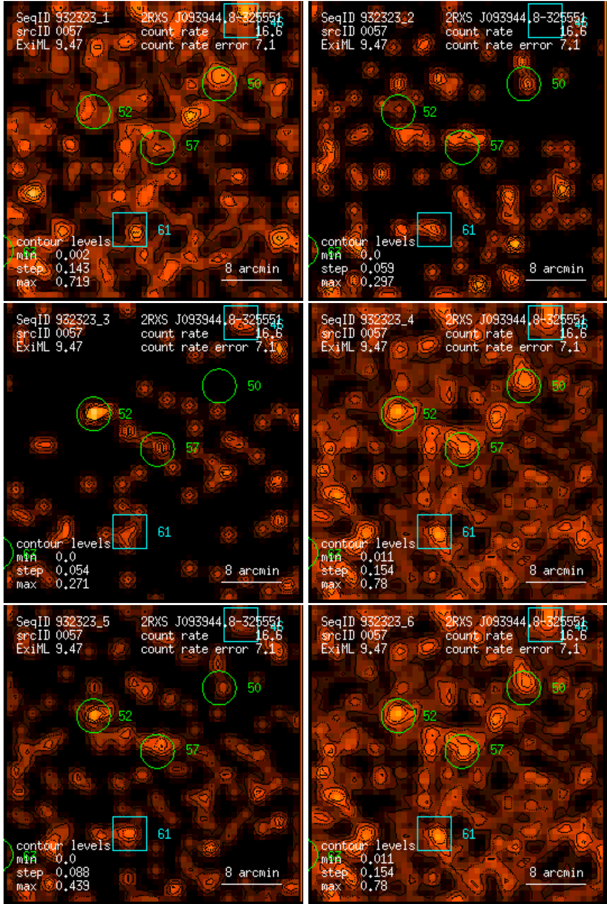
Figure 57: RASS 932323: detection 0057: band rate images, Gaussian filter: (1) PSPC channels 11 – 41, (2) 52 – 90, (3) 91 – 201, (4) 11 – 235, (5) 52 – 201, (6) 11 – 201. Broad band rates in counts/ks. Band rate contour levels in counts/ks/arcmin 2 .
