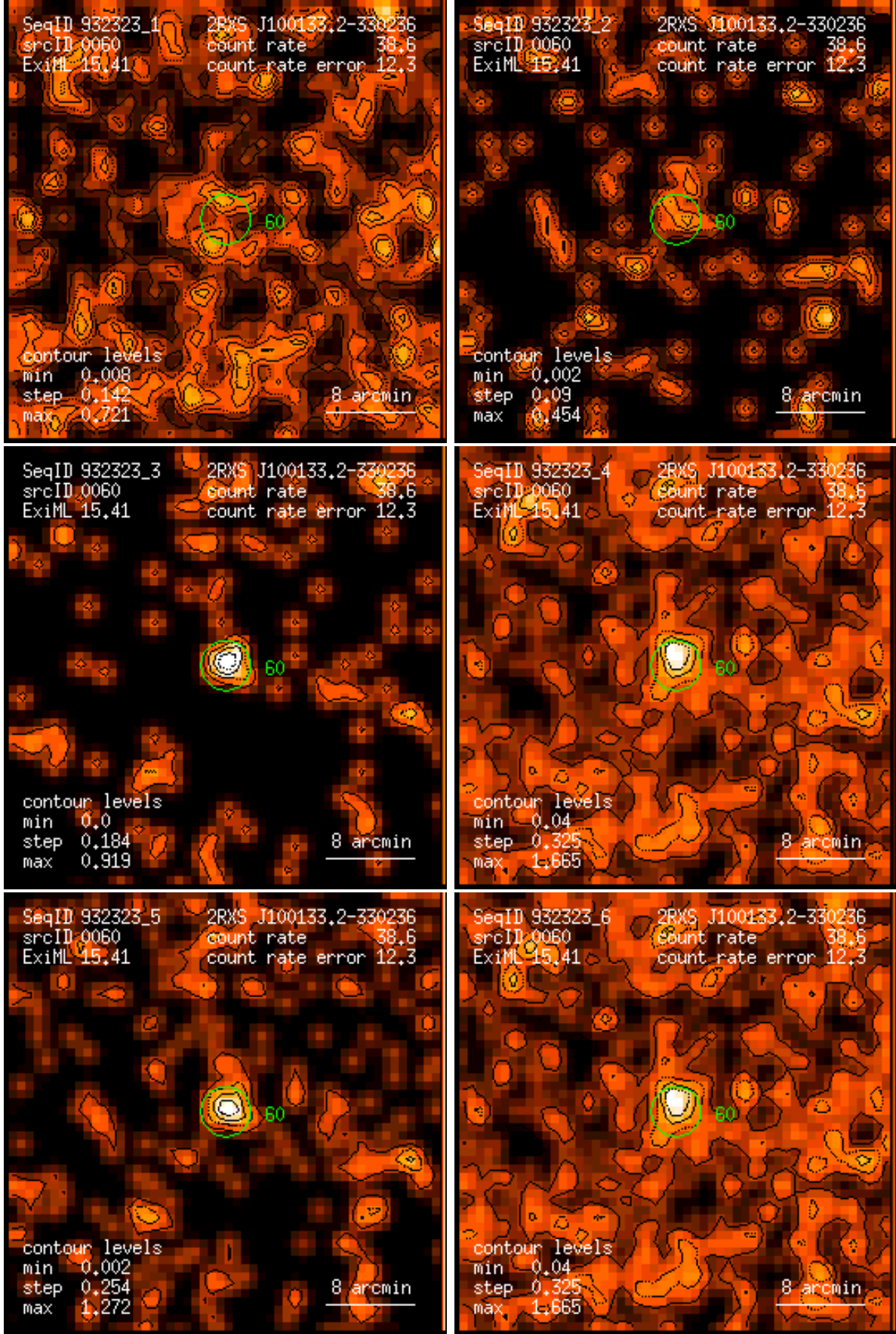
Figure 60: RASS 932323: detection 0060: band rate images, Gaussian filter: (1) PSPC channels 11 – 41, (2) 52 – 90, (3) 91 – 201, (4) 11 – 235, (5) 52 – 201, (6) 11 – 201. Broad band rates in counts/ks. Band rate contour levels in counts/ks/arcmin 2 .
