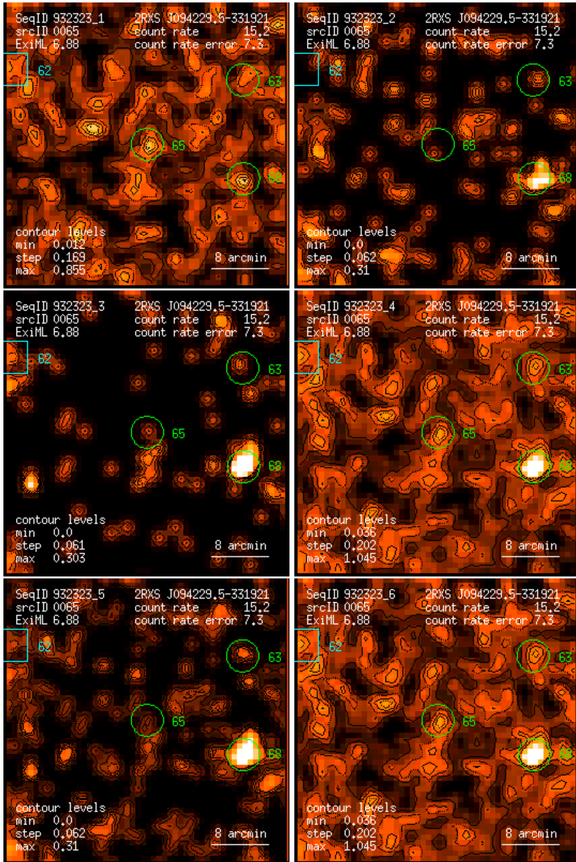
Figure 65: RASS 932323: detection 0065: band rate images, Gaussian filter: (1) PSPC channels 11 – 41, (2) 52 – 90, (3) 91 – 201, (4) 11 – 235, (5) 52 – 201, (6) 11 – 201. Broad band rates in counts/ks. Band rate contour levels in counts/ks/arcmin 2 .
