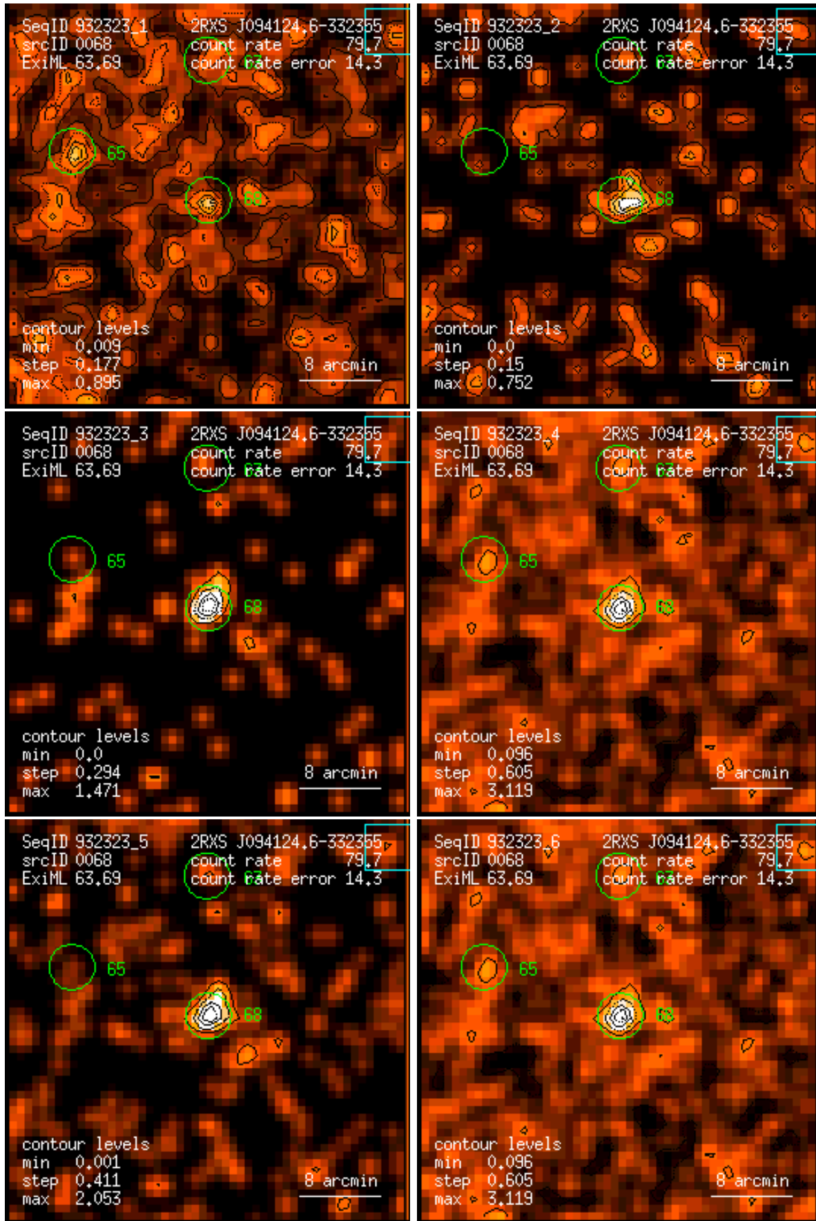
Figure 68: RASS 932323: detection 0068: band rate images, Gaussian filter: (1) PSPC channels 11 – 41, (2) 52 – 90, (3) 91 – 201, (4) 11 – 235, (5) 52 – 201, (6) 11 – 201. Broad band rates in counts/ks. Band rate contour levels in counts/ks/arcmin 2 .
