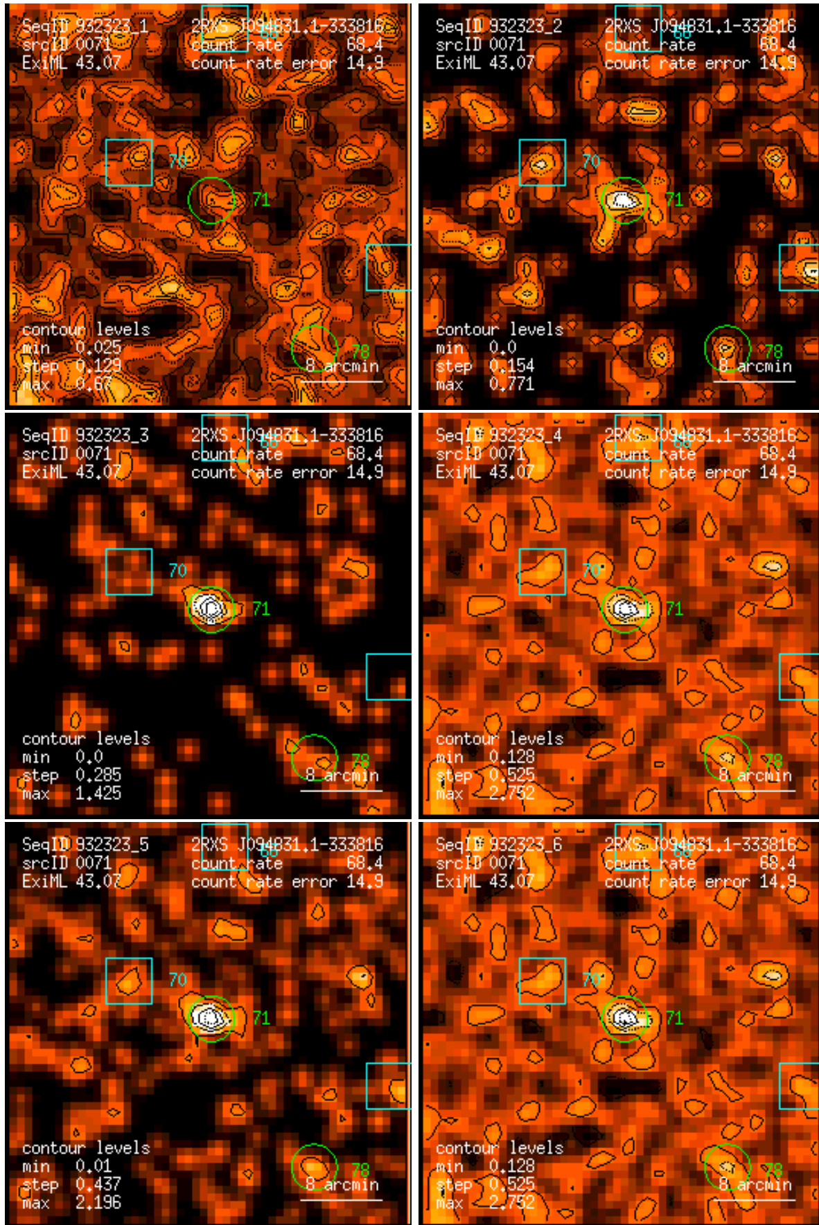
Figure 71: RASS 932323: detection 0071: band rate images, Gaussian filter: (1) PSPC channels 11 – 41, (2) 52 – 90, (3) 91 – 201, (4) 11 – 235, (5) 52 – 201, (6) 11 – 201. Broad band rates in counts/ks. Band rate contour levels in counts/ks/arcmin 2 .
