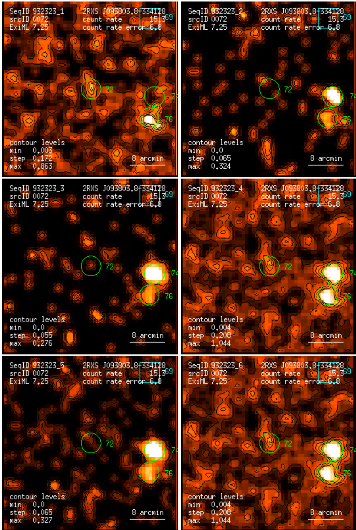
Figure 72: RASS 932323: detection 0072: band rate images, Gaussian filter: (1) PSPC channels 11 – 41, (2) 52 – 90, (3) 91 – 201, (4) 11 – 235, (5) 52 – 201, (6) 11 – 201. Broad band rates in counts/ks. Band rate contour levels in counts/ks/arcmin 2 .
