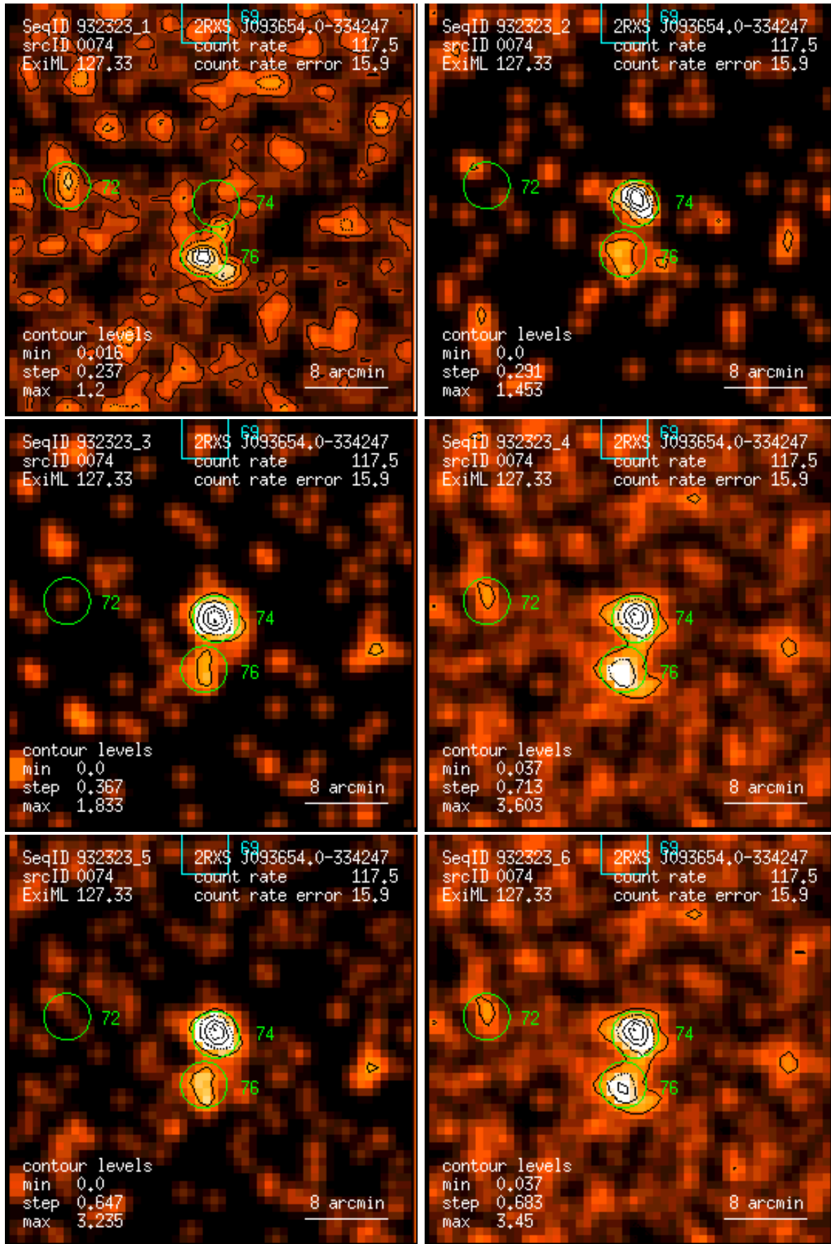
Figure 74: RASS 932323: detection 0074: band rate images, Gaussian filter: (1) PSPC channels 11 – 41, (2) 52 – 90, (3) 91 – 201, (4) 11 – 235, (5) 52 – 201, (6) 11 – 201. Broad band rates in counts/ks. Band rate contour levels in counts/ks/arcmin 2 .
