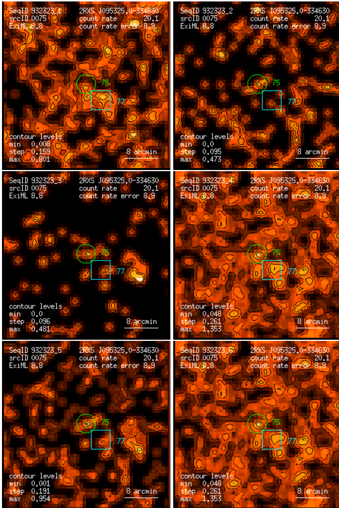
Figure 75: RASS 932323: detection 0075: band rate images, Gaussian filter: (1) PSPC channels 11 – 41, (2) 52 – 90, (3) 91 – 201, (4) 11 – 235, (5) 52 – 201, (6) 11 – 201. Broad band rates in counts/ks. Band rate contour levels in counts/ks/arcmin 2 .
