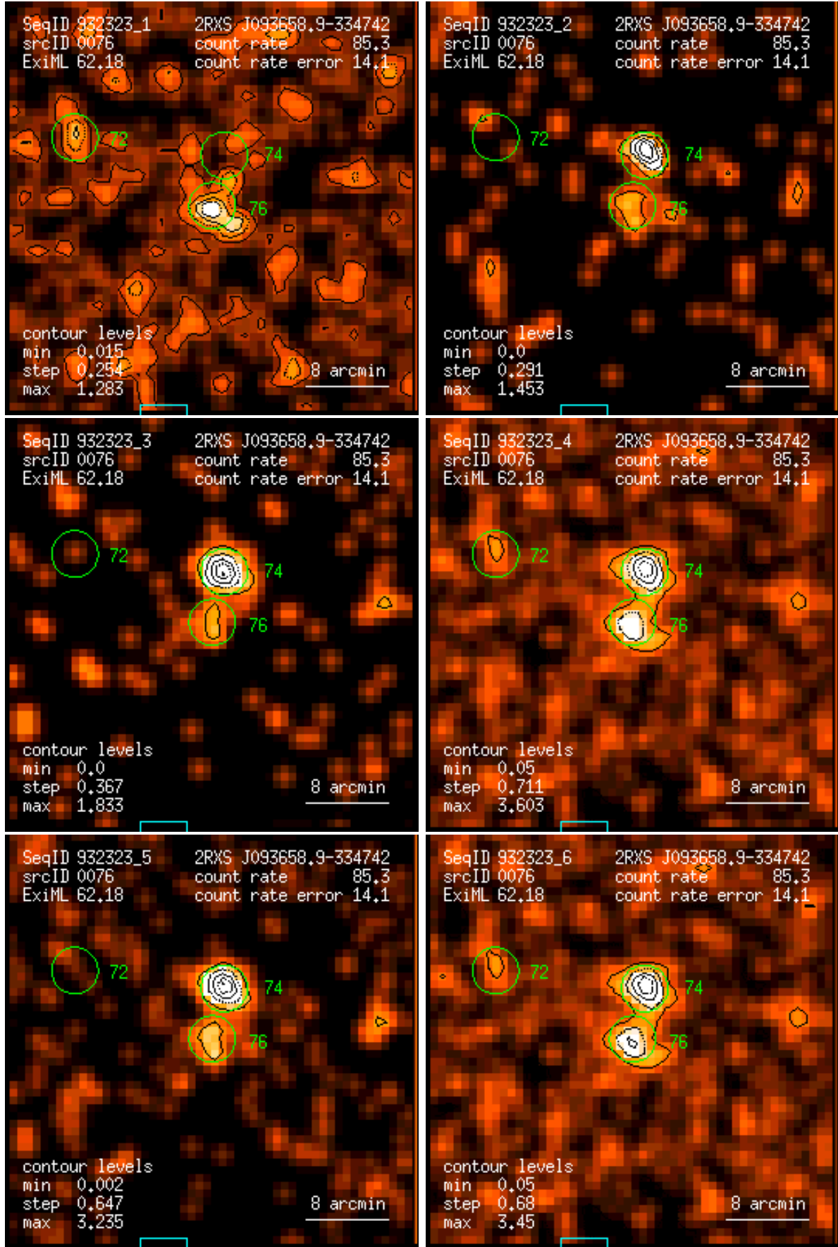
Figure 76: RASS 932323: detection 0076: band rate images, Gaussian filter: (1) PSPC channels 11 – 41, (2) 52 – 90, (3) 91 – 201, (4) 11 – 235, (5) 52 – 201, (6) 11 – 201. Broad band rates in counts/ks. Band rate contour levels in counts/ks/arcmin 2 .
