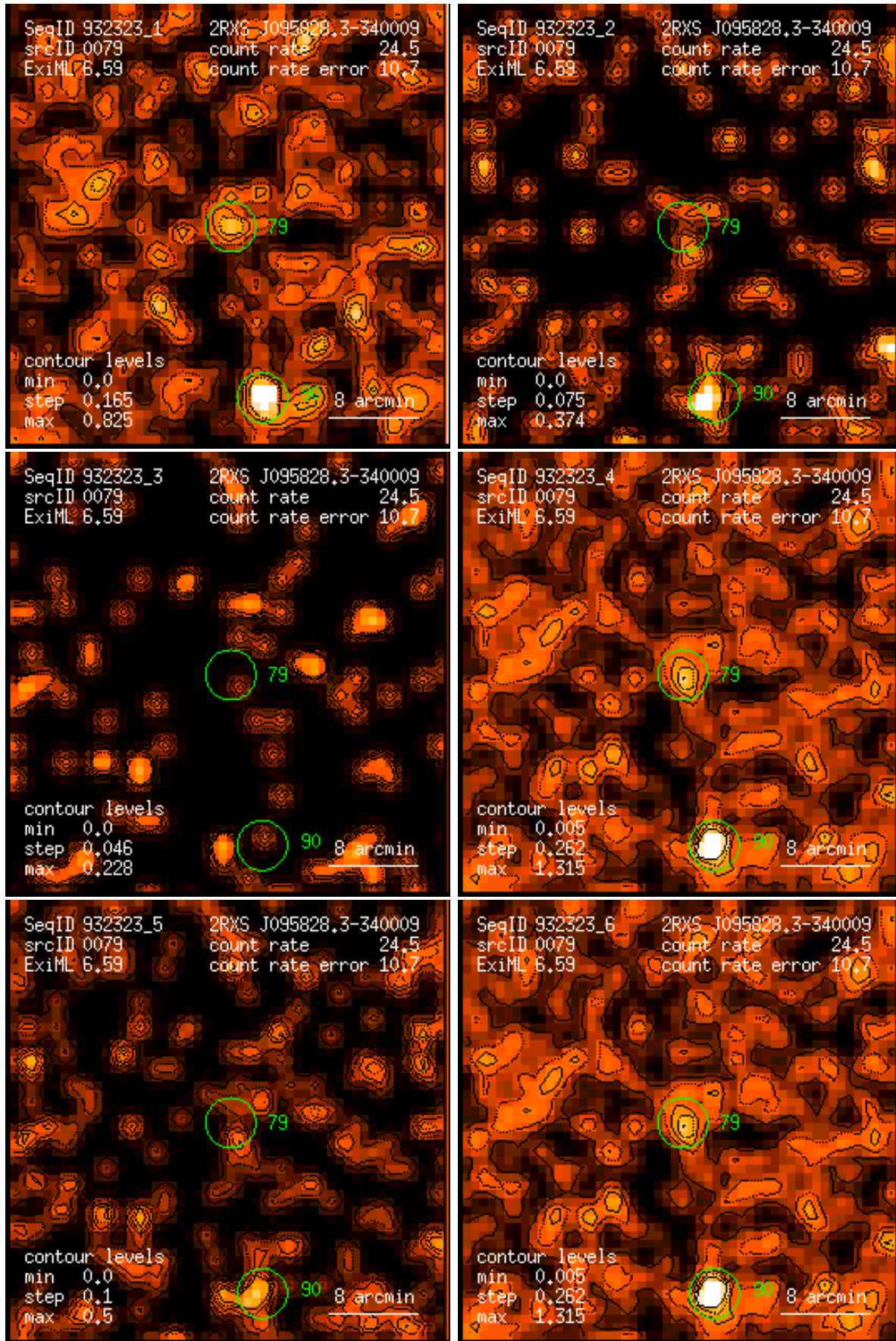
Figure 79: RASS 932323: detection 0079: band rate images, Gaussian filter: (1) PSPC channels 11 – 41, (2) 52 – 90, (3) 91 – 201, (4) 11 – 235, (5) 52 – 201, (6) 11 – 201. Broad band rates in counts/ks. Band rate contour levels in counts/ks/arcmin 2 .
