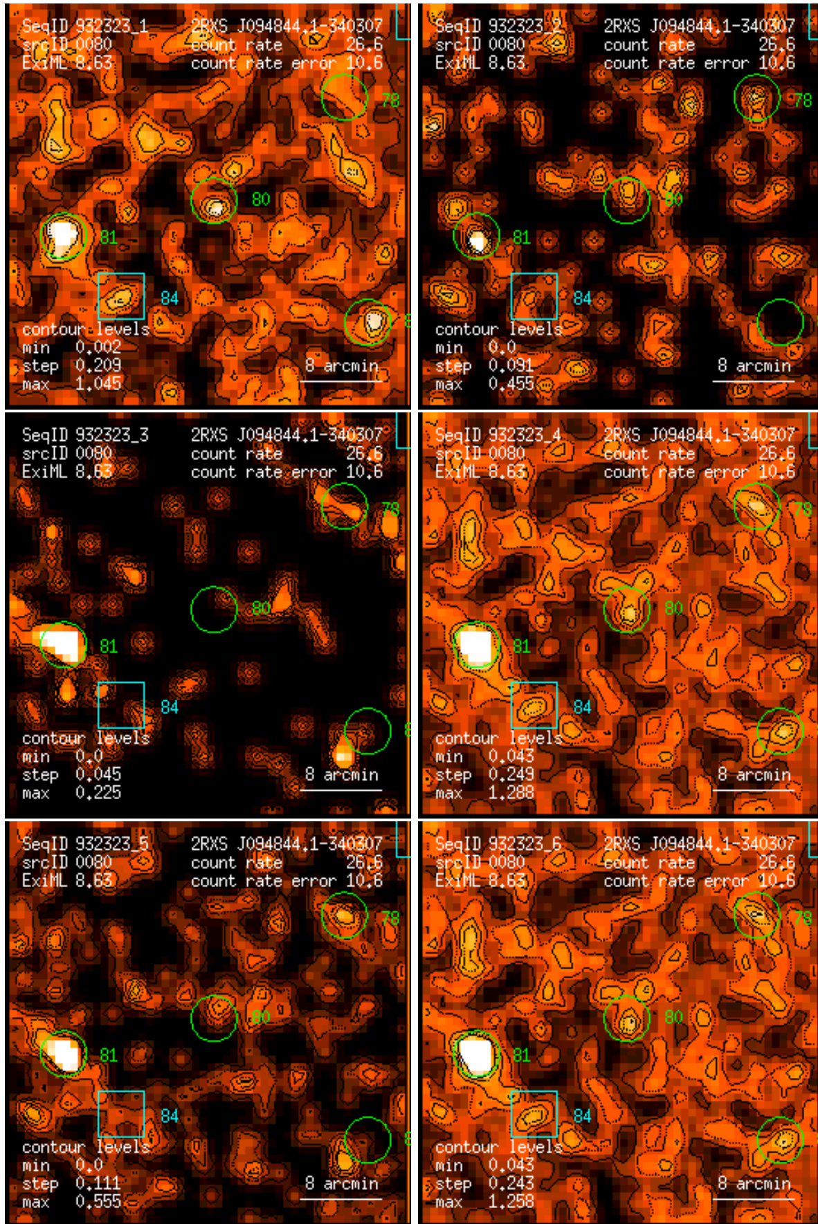
Figure 80: RASS 932323: detection 0080: band rate images, Gaussian filter: (1) PSPC channels 11 – 41, (2) 52 – 90, (3) 91 – 201, (4) 11 – 235, (5) 52 – 201, (6) 11 – 201. Broad band rates in counts/ks. Band rate contour levels in counts/ks/arcmin 2 .
