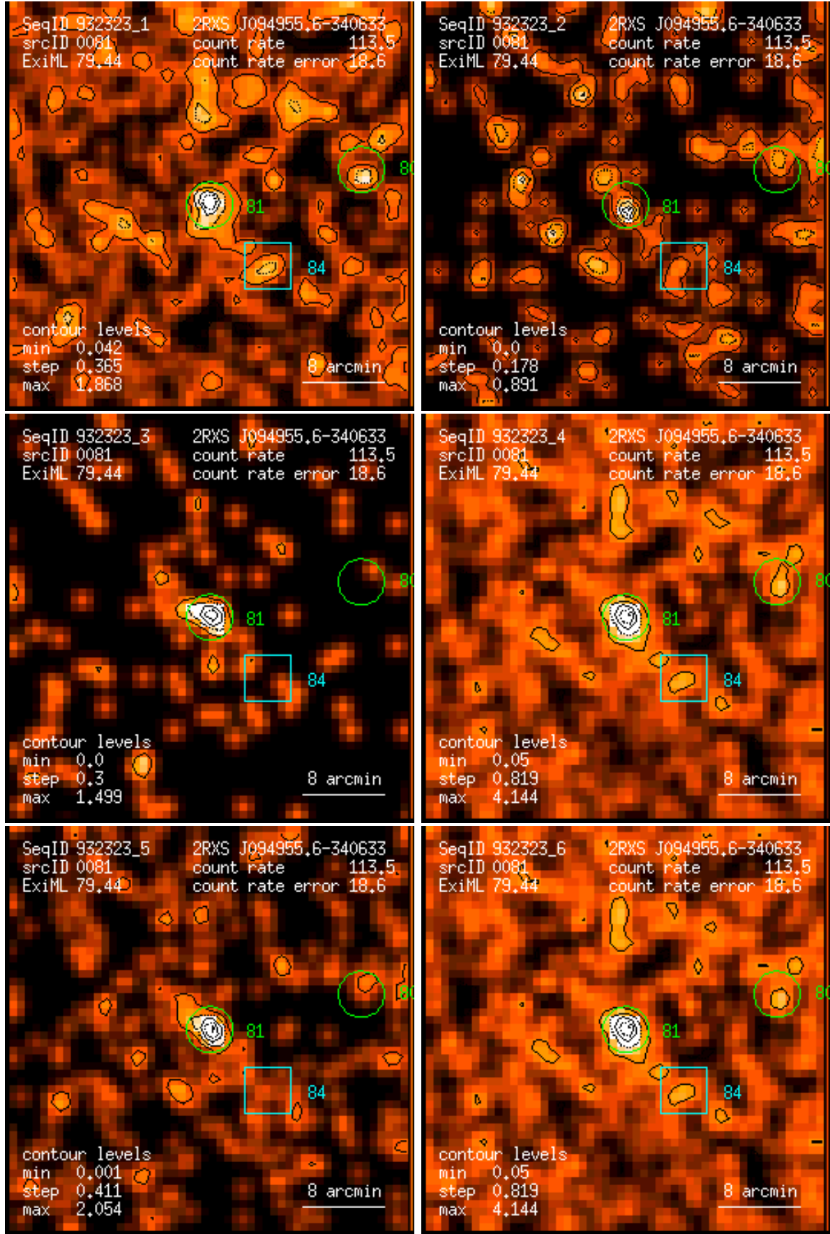
Figure 81: RASS 932323: detection 0081: band rate images, Gaussian filter: (1) PSPC channels 11 – 41, (2) 52 – 90, (3) 91 – 201, (4) 11 – 235, (5) 52 – 201, (6) 11 – 201. Broad band rates in counts/ks. Band rate contour levels in counts/ks/arcmin 2 .
