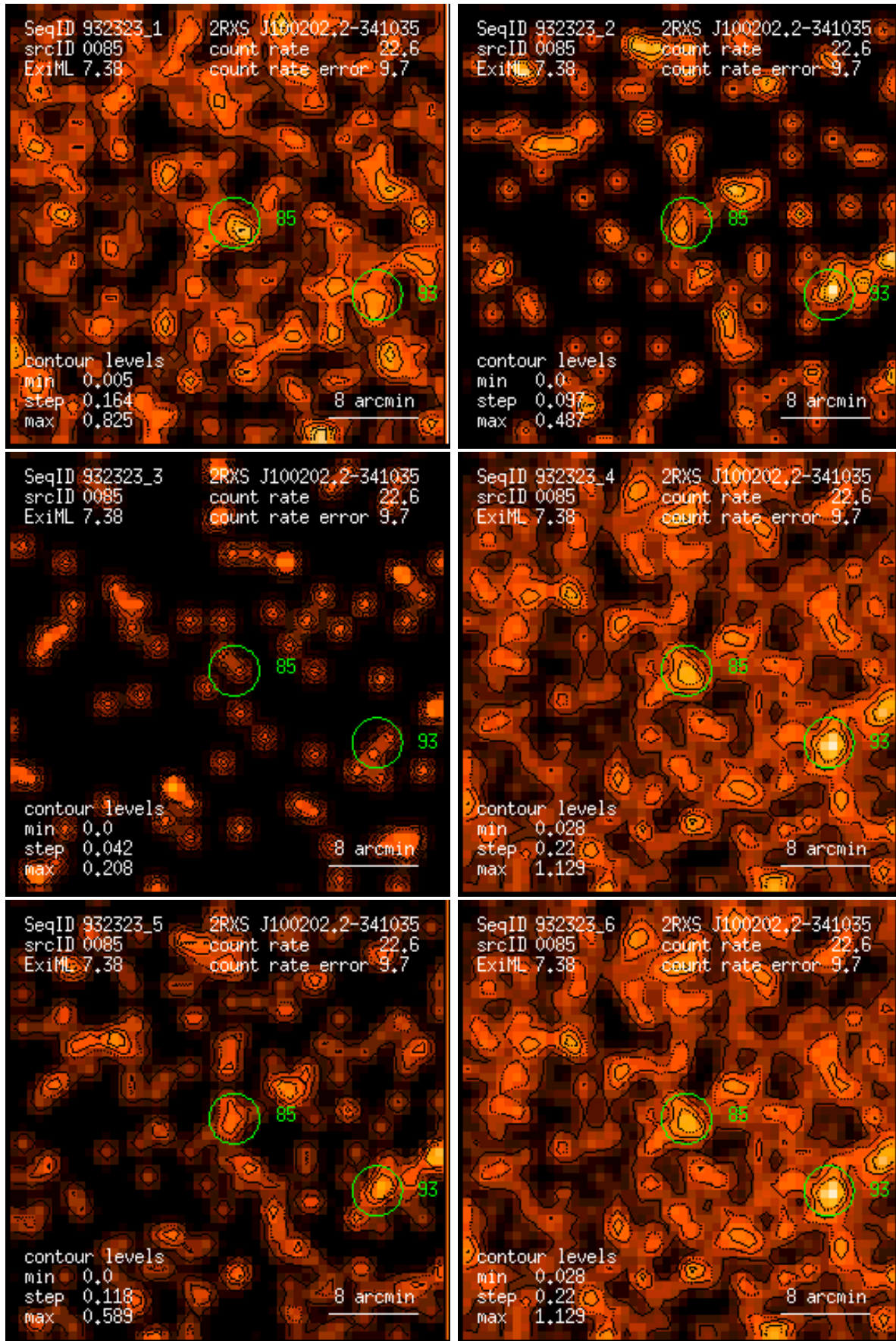
Figure 85: RASS 932323: detection 0085: band rate images, Gaussian filter: (1) PSPC channels 11 – 41, (2) 52 – 90, (3) 91 – 201, (4) 11 – 235, (5) 52 – 201, (6) 11 – 201. Broad band rates in counts/ks. Band rate contour levels in counts/ks/arcmin 2 .
