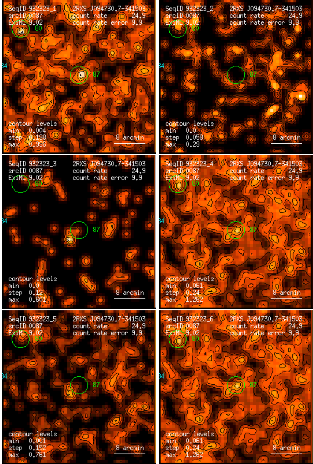
Figure 87: RASS 932323: detection 0087: band rate images, Gaussian filter: (1) PSPC channels 11 – 41, (2) 52 – 90, (3) 91 – 201, (4) 11 – 235, (5) 52 – 201, (6) 11 – 201. Broad band rates in counts/ks. Band rate contour levels in counts/ks/arcmin 2 .
