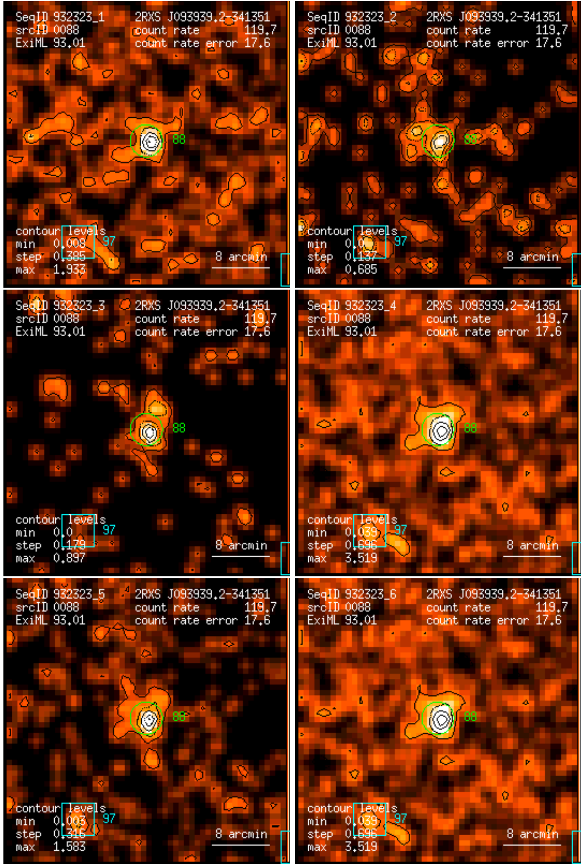
Figure 88: RASS 932323: detection 0088: band rate images, Gaussian filter: (1) PSPC channels 11 – 41, (2) 52 – 90, (3) 91 – 201, (4) 11 – 235, (5) 52 – 201, (6) 11 – 201. Broad band rates in counts/ks. Band rate contour levels in counts/ks/arcmin 2 .
