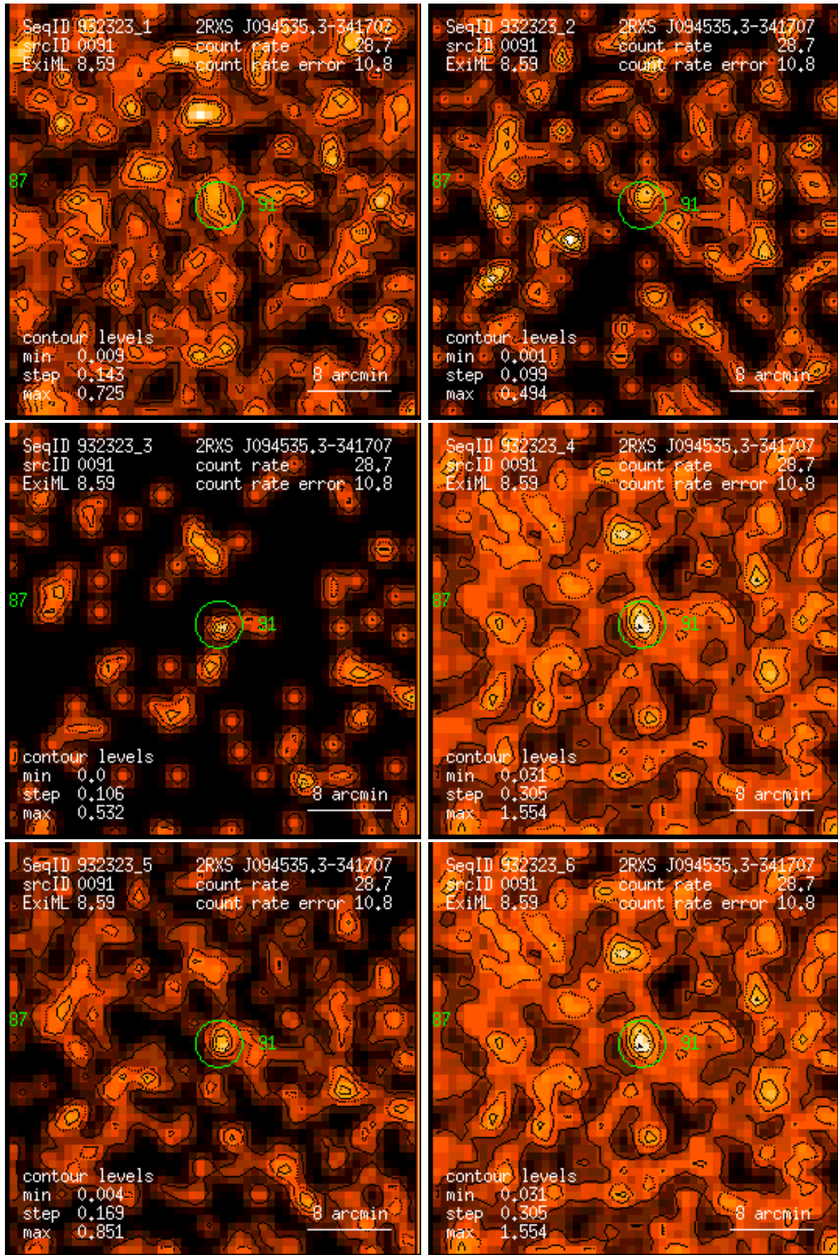
Figure 91: RASS 932323: detection 0091: band rate images, Gaussian filter: (1) PSPC channels 11 – 41, (2) 52 – 90, (3) 91 – 201, (4) 11 – 235, (5) 52 – 201, (6) 11 – 201. Broad band rates in counts/ks. Band rate contour levels in counts/ks/arcmin 2 .
