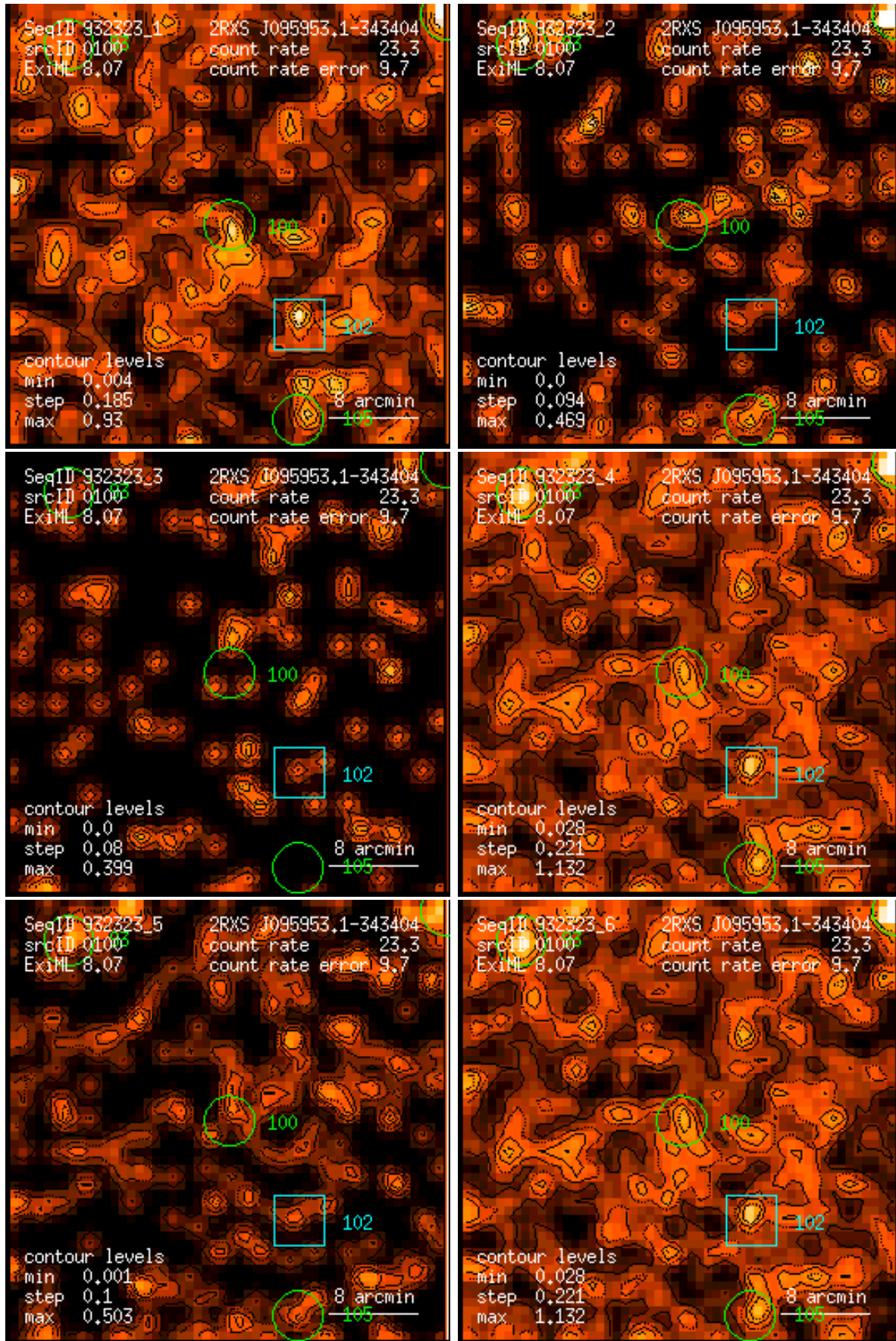
Figure 100: RASS 932323: detection 0100: band rate images, Gaussian filter: (1) PSPC channels 11 – 41, (2) 52 – 90, (3) 91 – 201, (4) 11 – 235, (5) 52 – 201, (6) 11 – 201. Broad band rates in counts/ks. Band rate contour levels in counts/ks/arcmin 2 .
