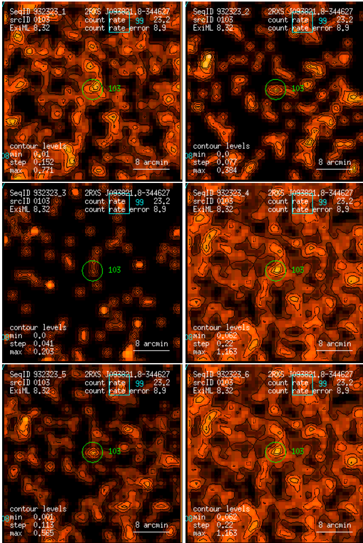
Figure 103: RASS 932323: detection 0103: band rate images, Gaussian filter: (1) PSPC channels 11 – 41, (2) 52 – 90, (3) 91 – 201, (4) 11 – 235, (5) 52 – 201, (6) 11 – 201. Broad band rates in counts/ks. Band rate contour levels in counts/ks/arcmin 2 .
